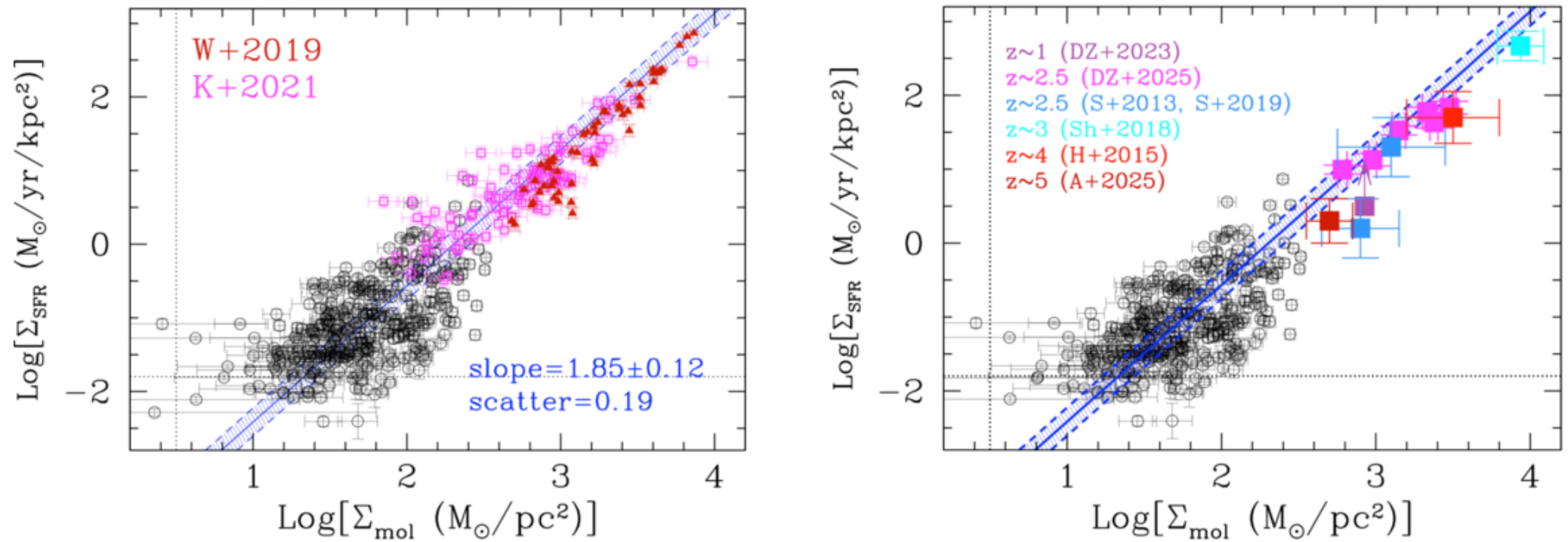
Figure 10. from Daniela Calzetti et al 2026 Astrophys. J. 1008 doi:10.3847/1538-4357/ae915b https://dx.doi.org/10.3847/1538-4357/ae915b © 2026. The Author(s). Published by the American Astronomical Society.
