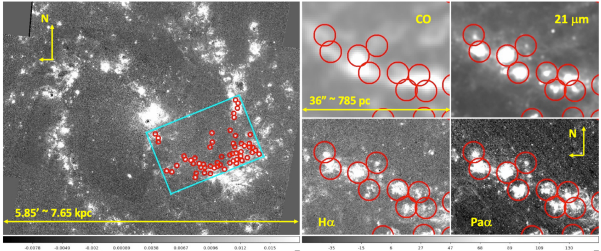
Figure 1. from Daniela Calzetti et al 2026 Astrophys. J. 1008 doi:10.3847/1538-4357/ae915b https://dx.doi.org/10.3847/1538-4357/ae915b © 2026. The Author(s). Published by the American Astronomical Society.
