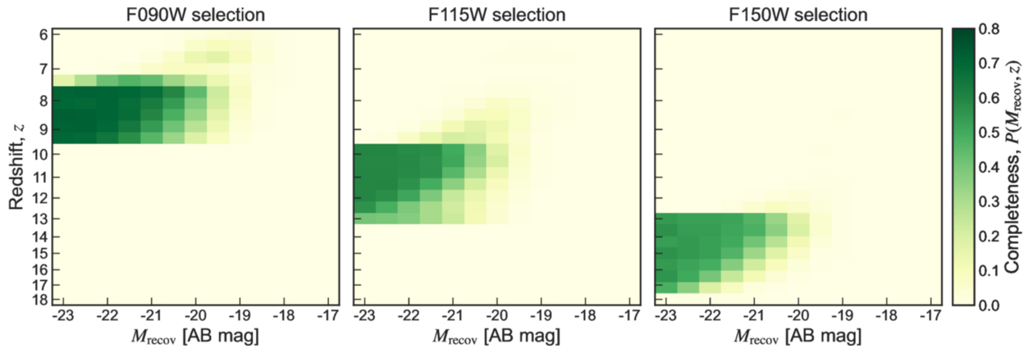
Figure 6. from Kimi C. Kreilgaard et al 2026 Astrophys. J. 1009 doi:10.3847/1538-4357/ae9152 https://dx.doi.org/10.3847/1538-4357/ae9152 © 2026. The Author(s). Published by the American Astronomical Society.
