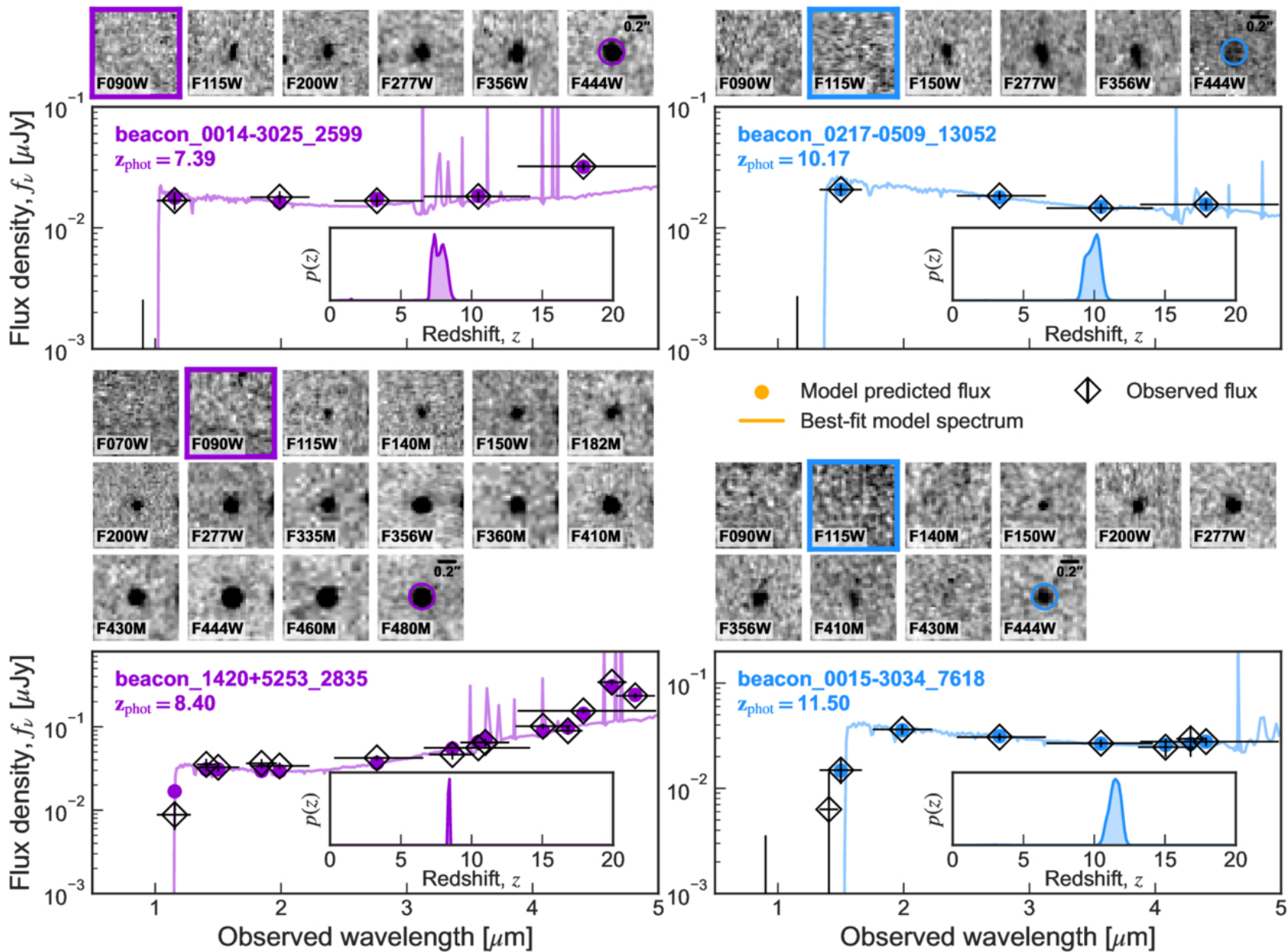
Figure 5. from Kimi C. Kreilgaard et al 2026 Astrophys. J. 1009 doi:10.3847/1538-4357/ae9152 https://dx.doi.org/10.3847/1538-4357/ae9152 © 2026. The Author(s). Published by the American Astronomical Society.
