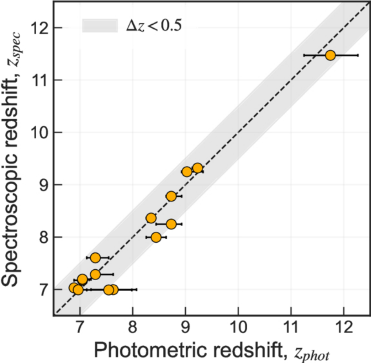
Figure 4. from Kimi C. Kreilgaard et al 2026 Astrophys. J. 1009 doi:10.3847/1538-4357/ae9152 https://dx.doi.org/10.3847/1538-4357/ae9152 © 2026. The Author(s). Published by the American Astronomical Society.
