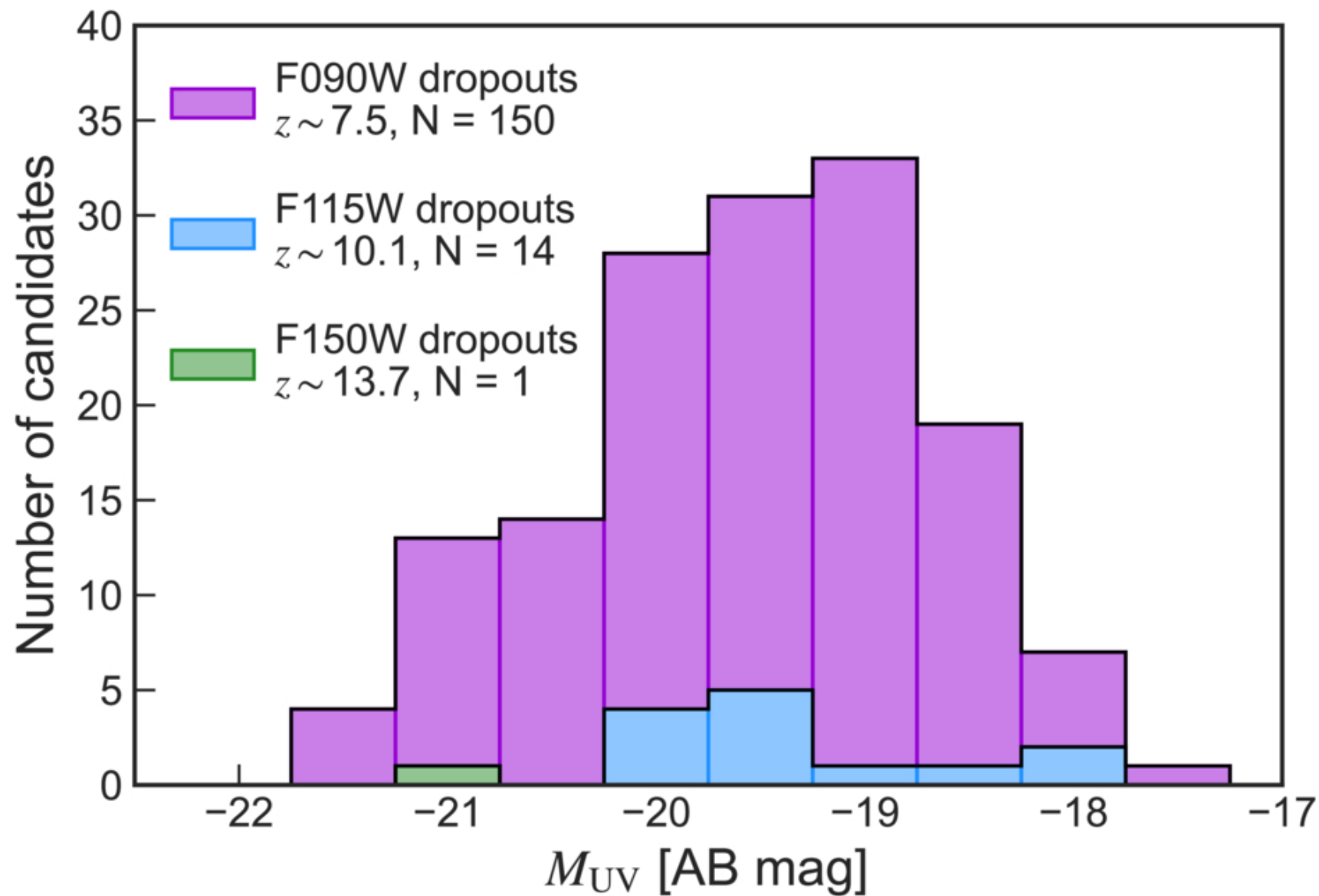
Figure 3. from Kimi C. Kreilgaard et al 2026 Astrophys. J. 1009 doi:10.3847/1538-4357/ae9152 https://dx.doi.org/10.3847/1538-4357/ae9152 © 2026. The Author(s). Published by the American Astronomical Society.
