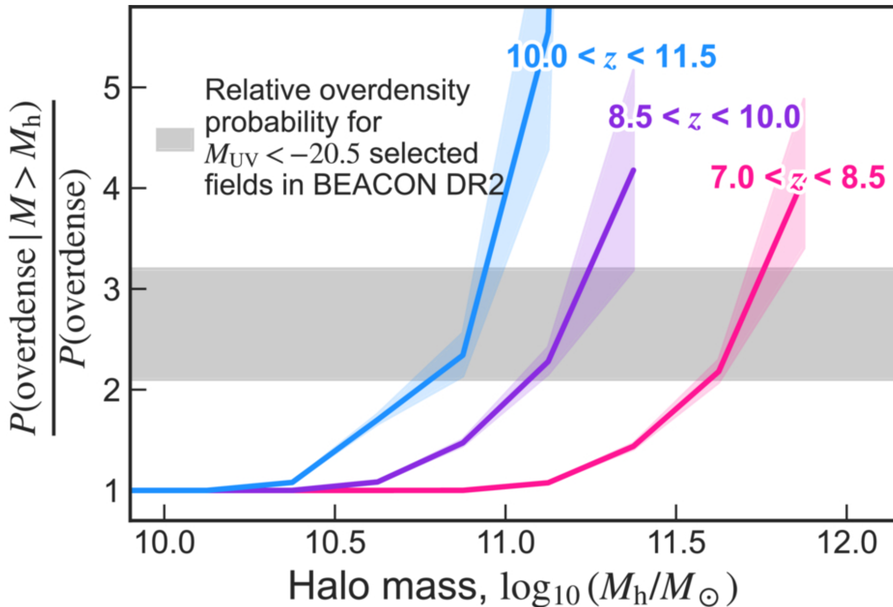
Figure 11. from Kimi C. Kreilgaard et al 2026 Astrophys. J. 1009 doi:10.3847/1538-4357/ae9152 https://dx.doi.org/10.3847/1538-4357/ae9152 © 2026. The Author(s). Published by the American Astronomical Society.
