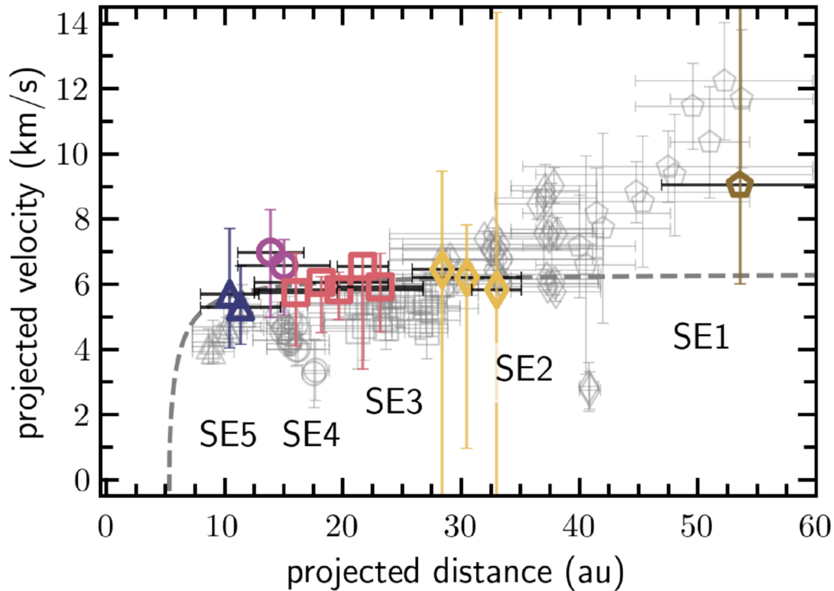
Figure 9. from Arcelia Hermosillo Ruiz et al 2026 Astrophys. J. 1008 doi:10.3847/1538-4357/ae90a7 https://dx.doi.org/10.3847/1538-4357/ae90a7 © 2026. The Author(s). Published by the American Astronomical Society.
