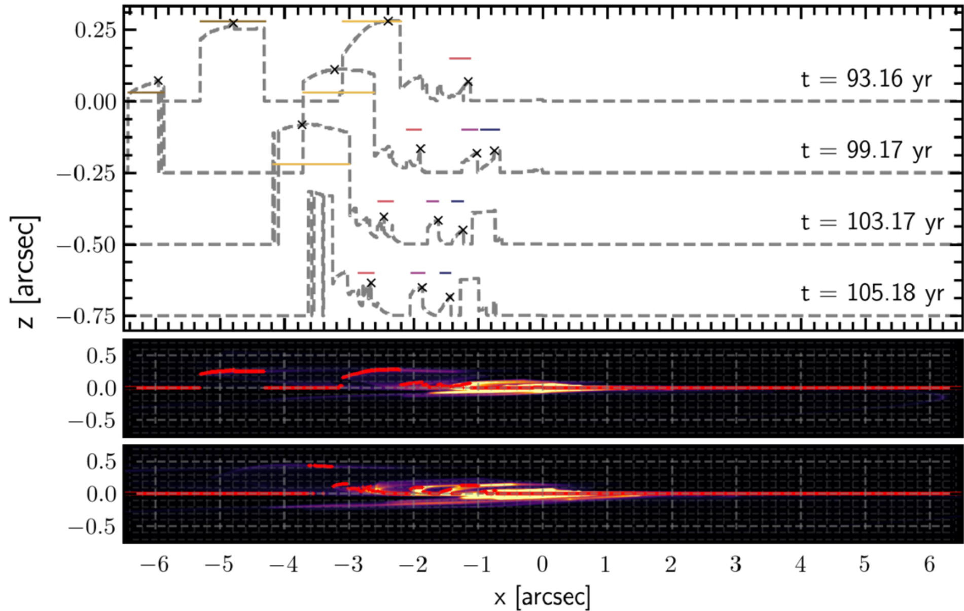
Figure 8. from Arcelia Hermosillo Ruiz et al 2026 Astrophys. J. 1008 doi:10.3847/1538-4357/ae90a7 https://dx.doi.org/10.3847/1538-4357/ae90a7 © 2026. The Author(s). Published by the American Astronomical Society.
