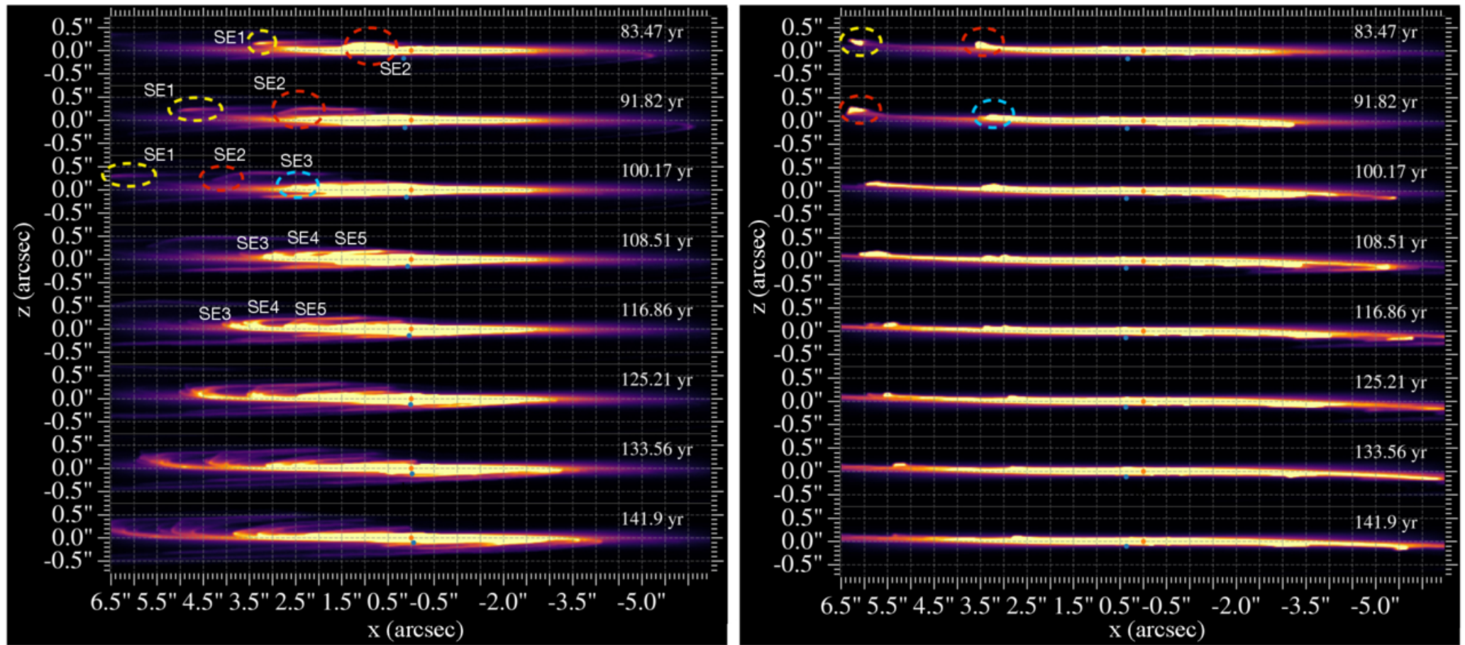
Figure 7. from Arcelia Hermosillo Ruiz et al 2026 Astrophys. J. 1008 doi:10.3847/1538-4357/ae90a7 https://dx.doi.org/10.3847/1538-4357/ae90a7 © 2026. The Author(s). Published by the American Astronomical Society.
