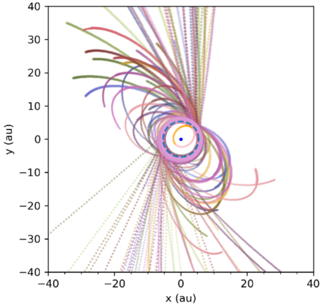
Figure 5. from Arcelia Hermosillo Ruiz et al 2026 Astrophys. J. 1008 doi:10.3847/1538-4357/ae90a7 https://dx.doi.org/10.3847/1538-4357/ae90a7 © 2026. The Author(s). Published by the American Astronomical Society.
