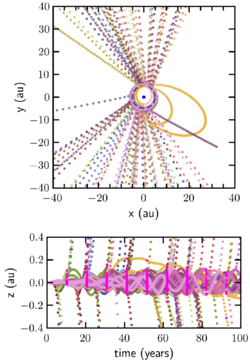
Figure 3. from Arcelia Hermosillo Ruiz et al 2026 Astrophys. J. 1008 doi:10.3847/1538-4357/ae90a7 https://dx.doi.org/10.3847/1538-4357/ae90a7 © 2026. The Author(s). Published by the American Astronomical Society.
