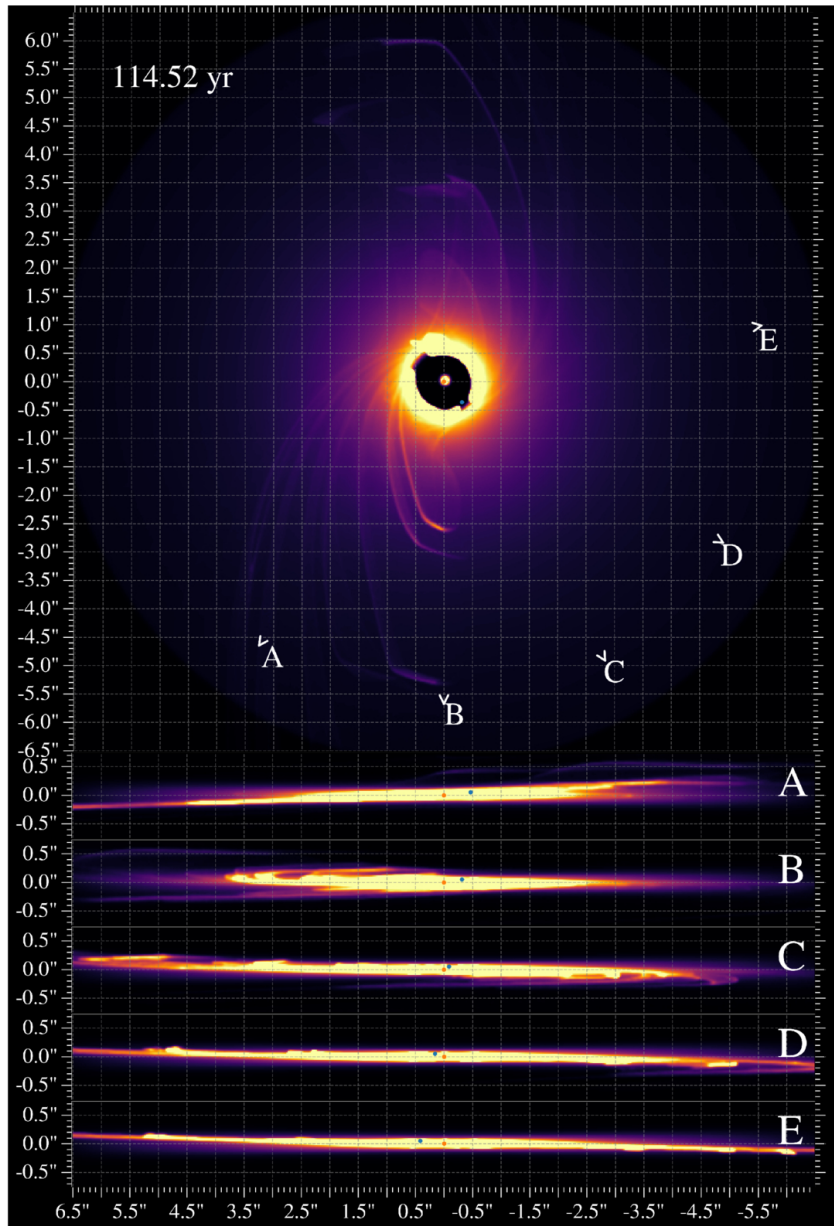
Figure 10. from Arcelia Hermosillo Ruiz et al 2026 Astrophys. J. 1008 doi:10.3847/1538-4357/ae90a7 https://dx.doi.org/10.3847/1538-4357/ae90a7 © 2026. The Author(s). Published by the American Astronomical Society.
