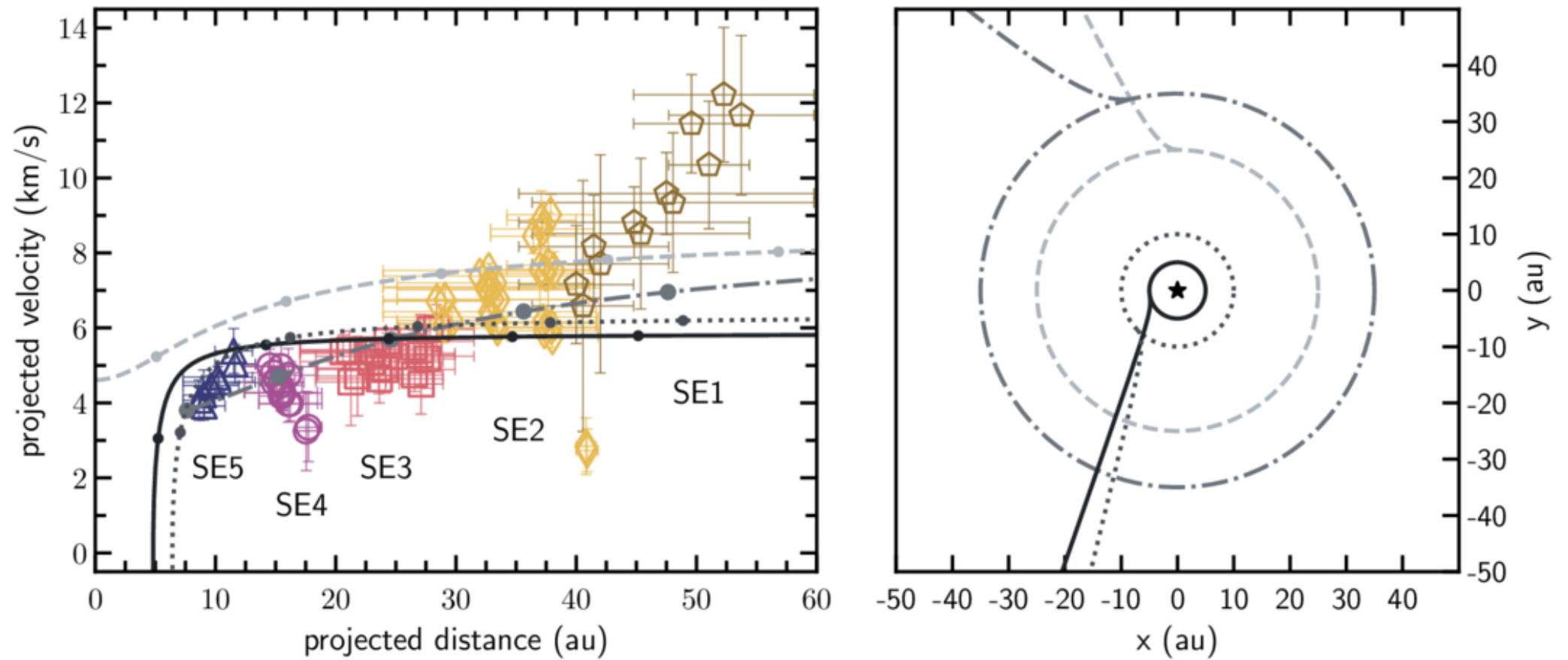
Figure 1. from Arcelia Hermosillo Ruiz et al 2026 Astrophys. J. 1008 doi:10.3847/1538-4357/ae90a7 https://dx.doi.org/10.3847/1538-4357/ae90a7 © 2026. The Author(s). Published by the American Astronomical Society.
