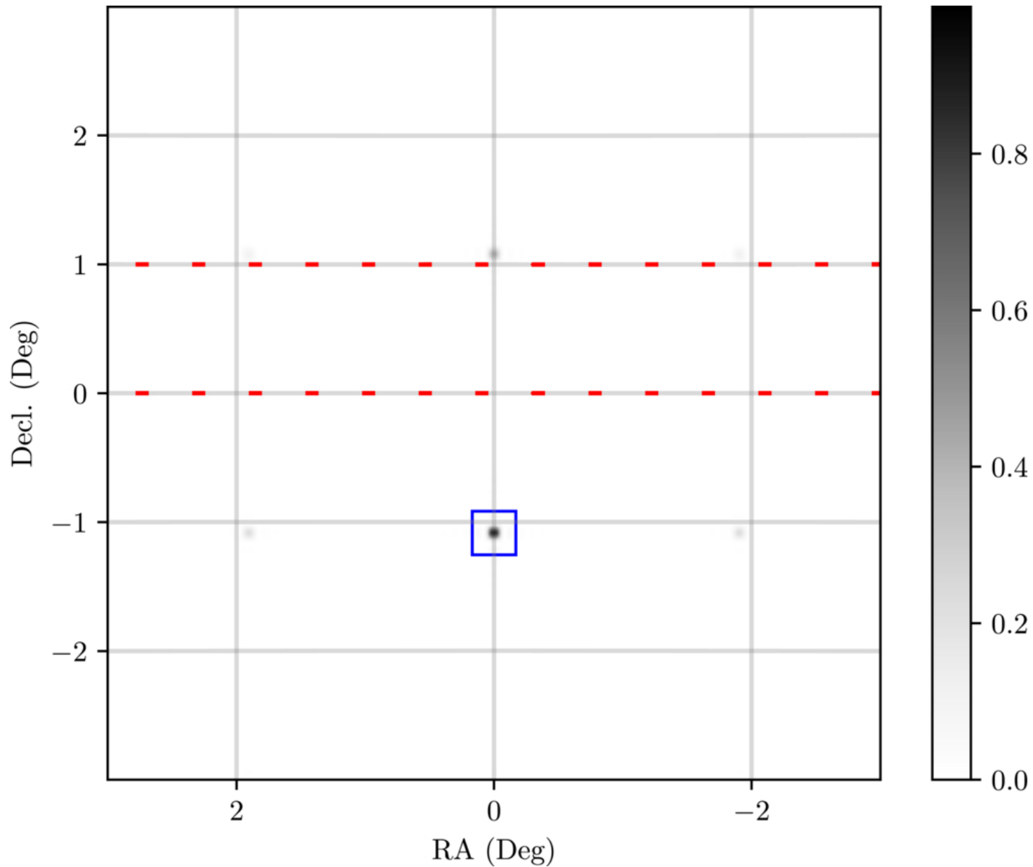
Figure 9. from Hans S. Hopkins et al 2026 Astrophys. J. 1008 doi:10.3847/1538-4357/ae9094 https://dx.doi.org/10.3847/1538-4357/ae9094 © 2026. The Author(s). Published by the American Astronomical Society.
