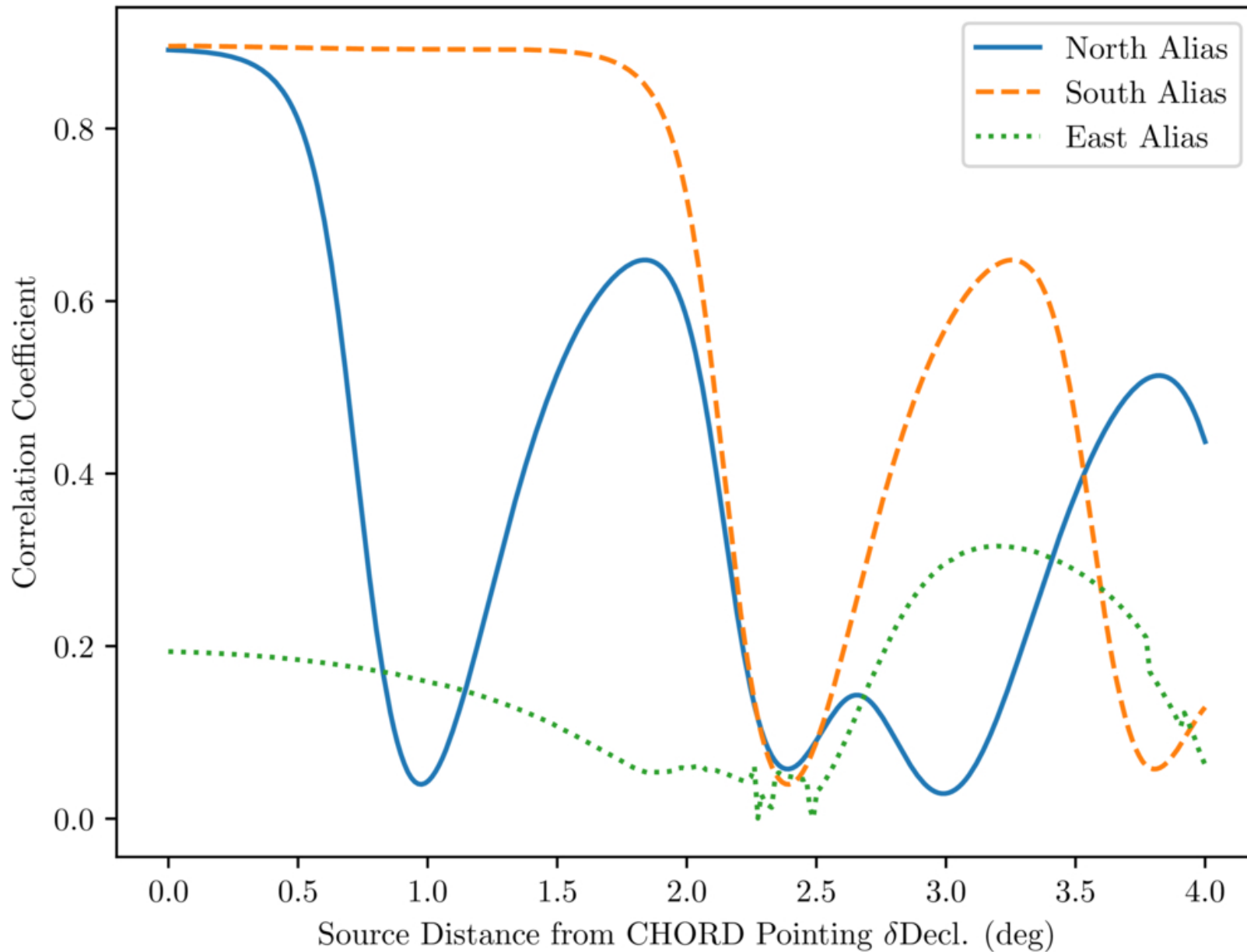
Figure 6. from Hans S. Hopkins et al 2026 Astrophys. J. 1008 doi:10.3847/1538-4357/ae9094 https://dx.doi.org/10.3847/1538-4357/ae9094 © 2026. The Author(s). Published by the American Astronomical Society.
