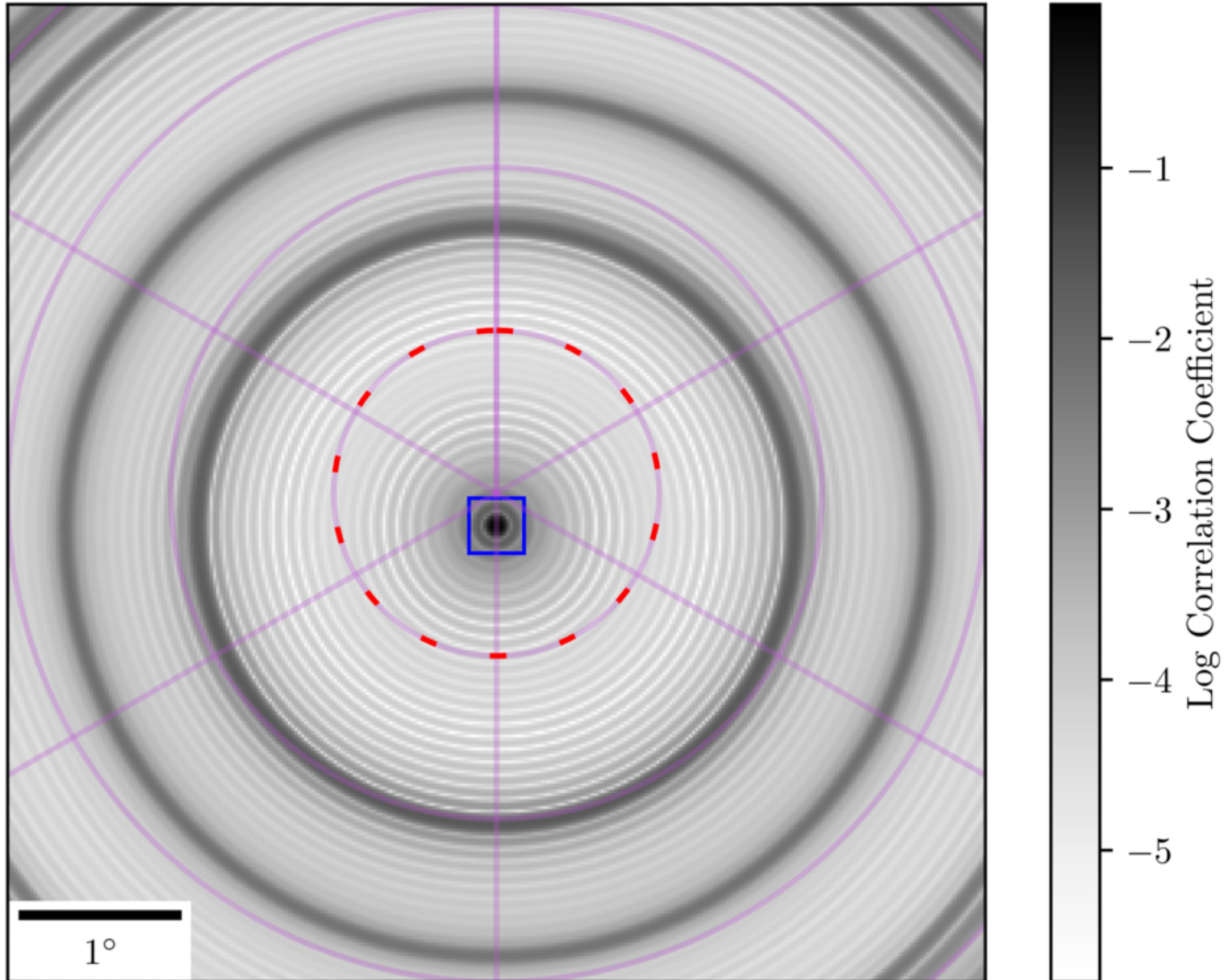
Figure 5. from Hans S. Hopkins et al 2026 Astrophys. J. 1008 doi:10.3847/1538-4357/ae9094 https://dx.doi.org/10.3847/1538-4357/ae9094 © 2026. The Author(s). Published by the American Astronomical Society.
