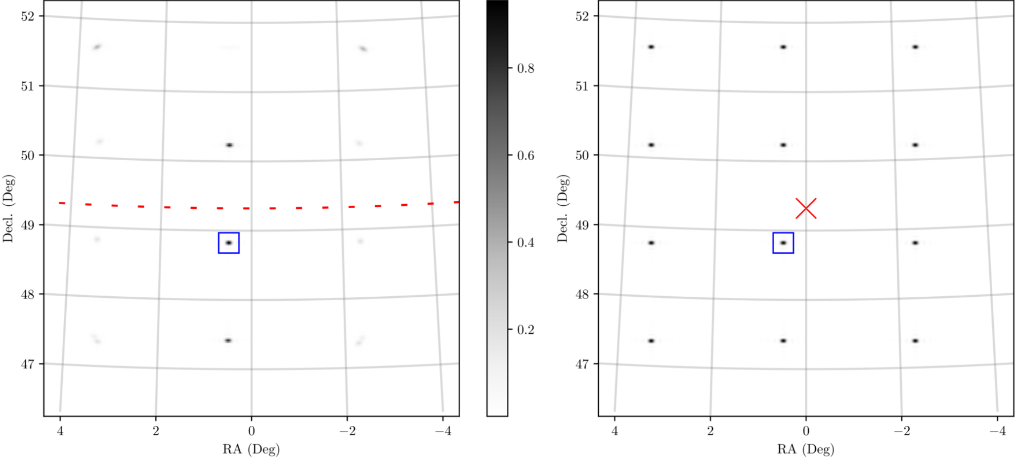
Figure 4. from Hans S. Hopkins et al 2026 Astrophys. J. 1008 doi:10.3847/1538-4357/ae9094 https://dx.doi.org/10.3847/1538-4357/ae9094 © 2026. The Author(s). Published by the American Astronomical Society.
