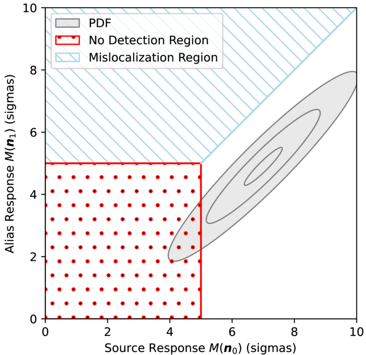
Figure 12. from Hans S. Hopkins et al 2026 Astrophys. J. 1008 doi:10.3847/1538-4357/ae9094 https://dx.doi.org/10.3847/1538-4357/ae9094 © 2026. The Author(s). Published by the American Astronomical Society.
