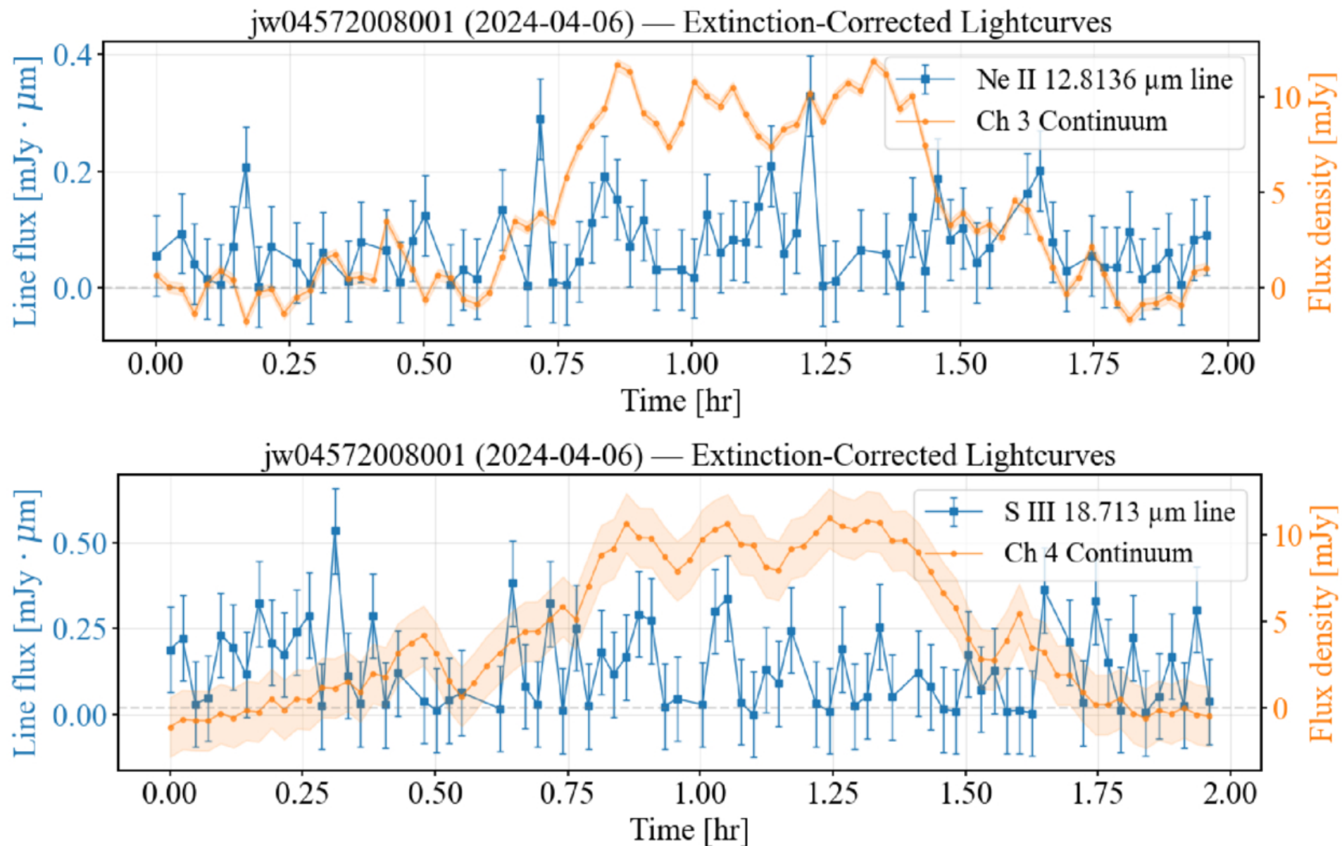
Figure 2. from Mayura Balakrishnan et al 2026 Astrophys. J. 1008 doi:10.3847/1538-4357/ae908b https://dx.doi.org/10.3847/1538-4357/ae908b © 2026. The Author(s). Published by the American Astronomical Society.
