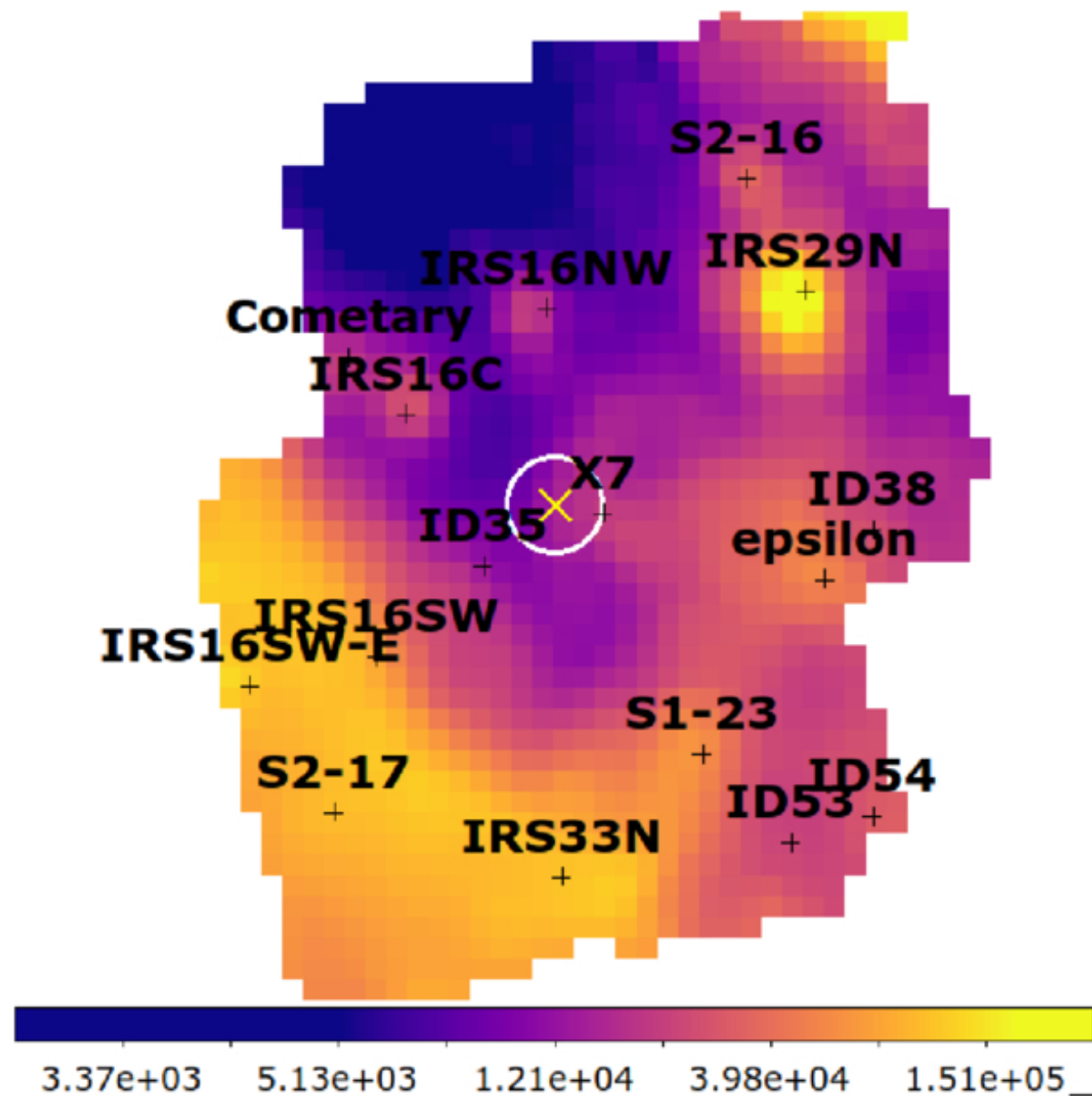
Figure 1. from Mayura Balakrishnan et al 2026 Astrophys. J. 1008 doi:10.3847/1538-4357/ae908b https://dx.doi.org/10.3847/1538-4357/ae908b © 2026. The Author(s). Published by the American Astronomical Society.
