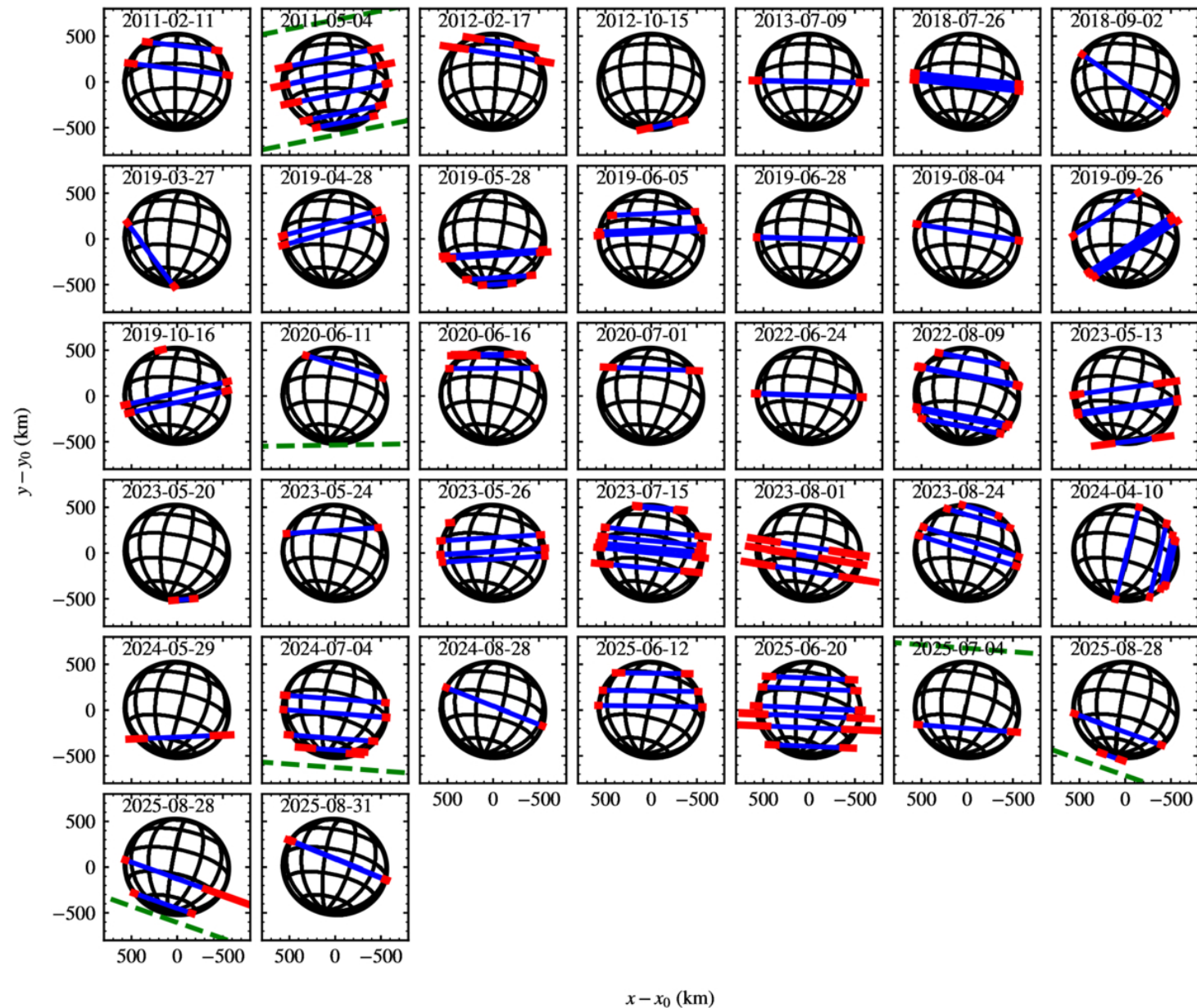
Figure 2. from Giuliano Margoti et al 2026 Astrophys. J. 1008 doi:10.3847/1538-4357/ae907e https://dx.doi.org/10.3847/1538-4357/ae907e © 2026. The Author(s). Published by the American Astronomical Society.
