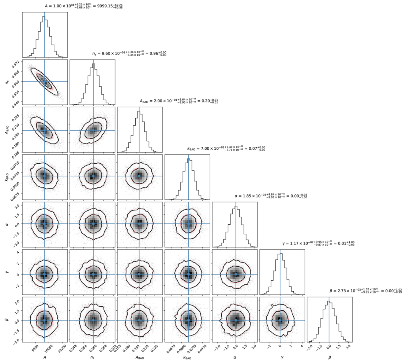
Figure 5. from Pierros Ntelis et al 2026 Astrophys. J. 1009 doi:10.3847/1538-4357/ae904d https://dx.doi.org/10.3847/1538-4357/ae904d © 2026. The Author(s). Published by the American Astronomical Society.
