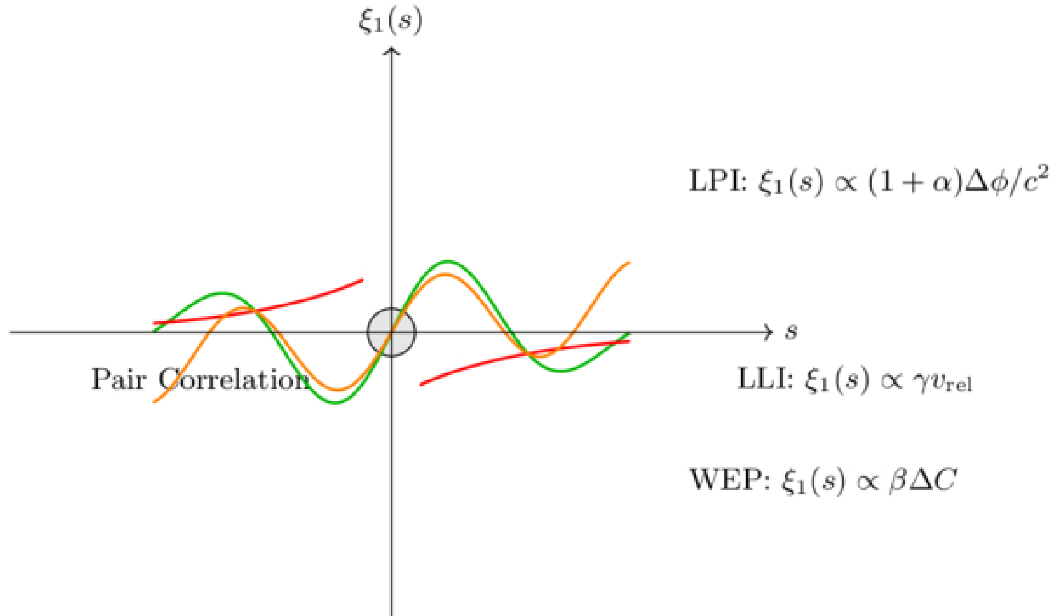
Figure 2. from Pierros Ntelis et al 2026 Astrophys. J. 1009 doi:10.3847/1538-4357/ae904d https://dx.doi.org/10.3847/1538-4357/ae904d © 2026. The Author(s). Published by the American Astronomical Society.
