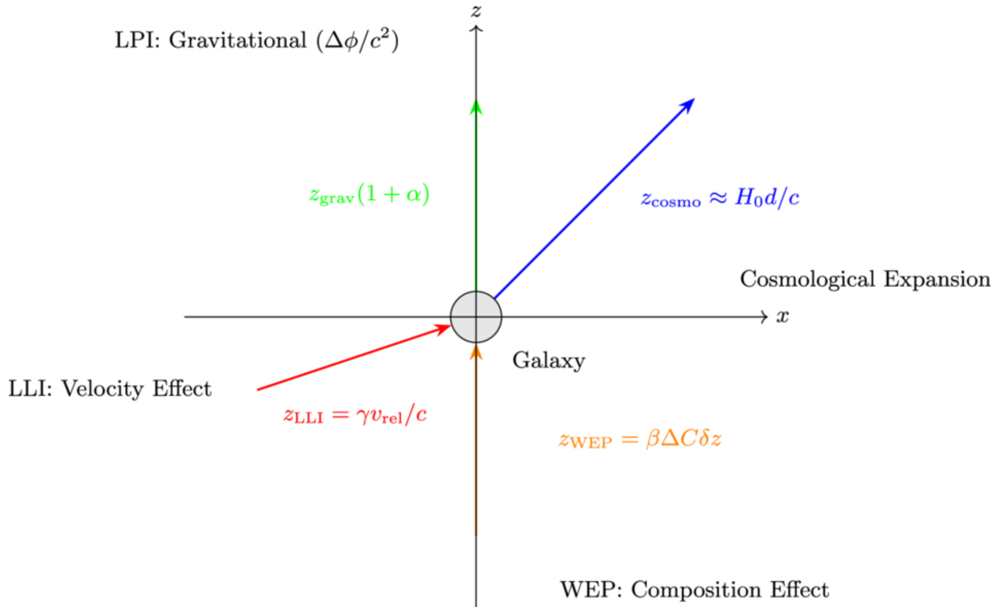
Figure 1. from Pierros Ntelis et al 2026 Astrophys. J. 1009 doi:10.3847/1538-4357/ae904d https://dx.doi.org/10.3847/1538-4357/ae904d © 2026. The Author(s). Published by the American Astronomical Society.
