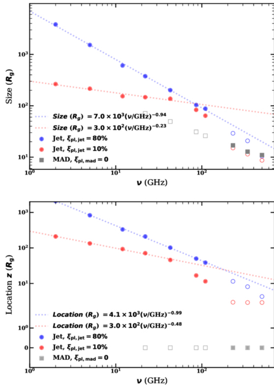
Figure 6. from Yue Xu et al 2026 Astrophys. J. 1007 doi:10.3847/1538-4357/ae8fd8 https://dx.doi.org/10.3847/1538-4357/ae8fd8 © 2026. The Author(s). Published by the American Astronomical Society.
