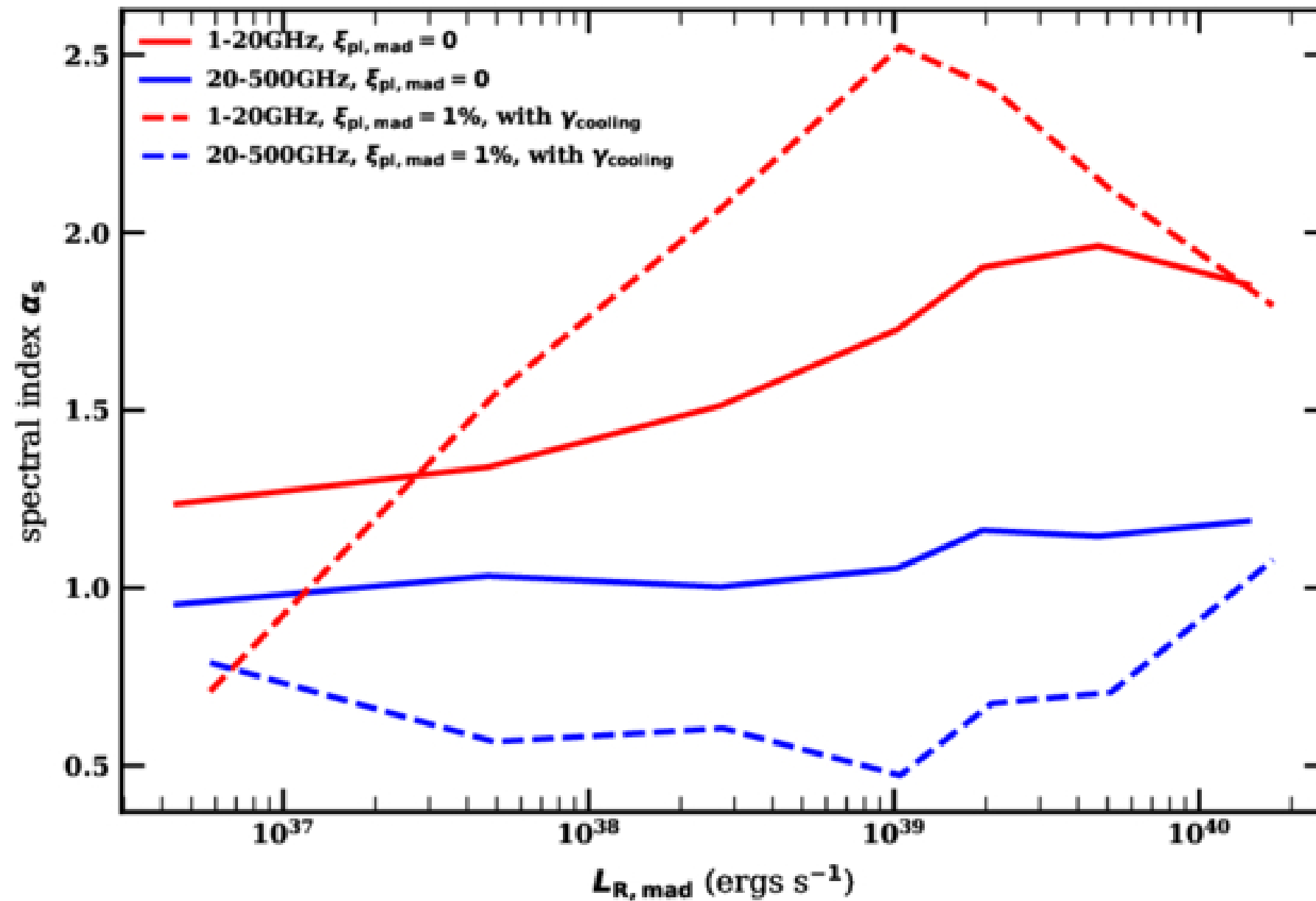
Figure 4. from Yue Xu et al 2026 Astrophys. J. 1007 doi:10.3847/1538-4357/ae8fd8 https://dx.doi.org/10.3847/1538-4357/ae8fd8 © 2026. The Author(s). Published by the American Astronomical Society.
