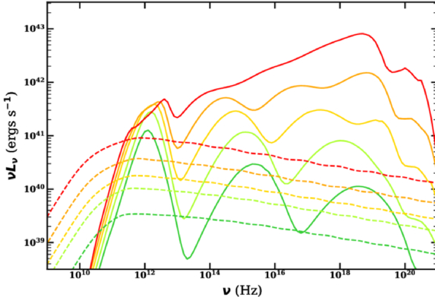
Figure 3. from Yue Xu et al 2026 Astrophys. J. 1007 doi:10.3847/1538-4357/ae8fd8 https://dx.doi.org/10.3847/1538-4357/ae8fd8 © 2026. The Author(s). Published by the American Astronomical Society.
