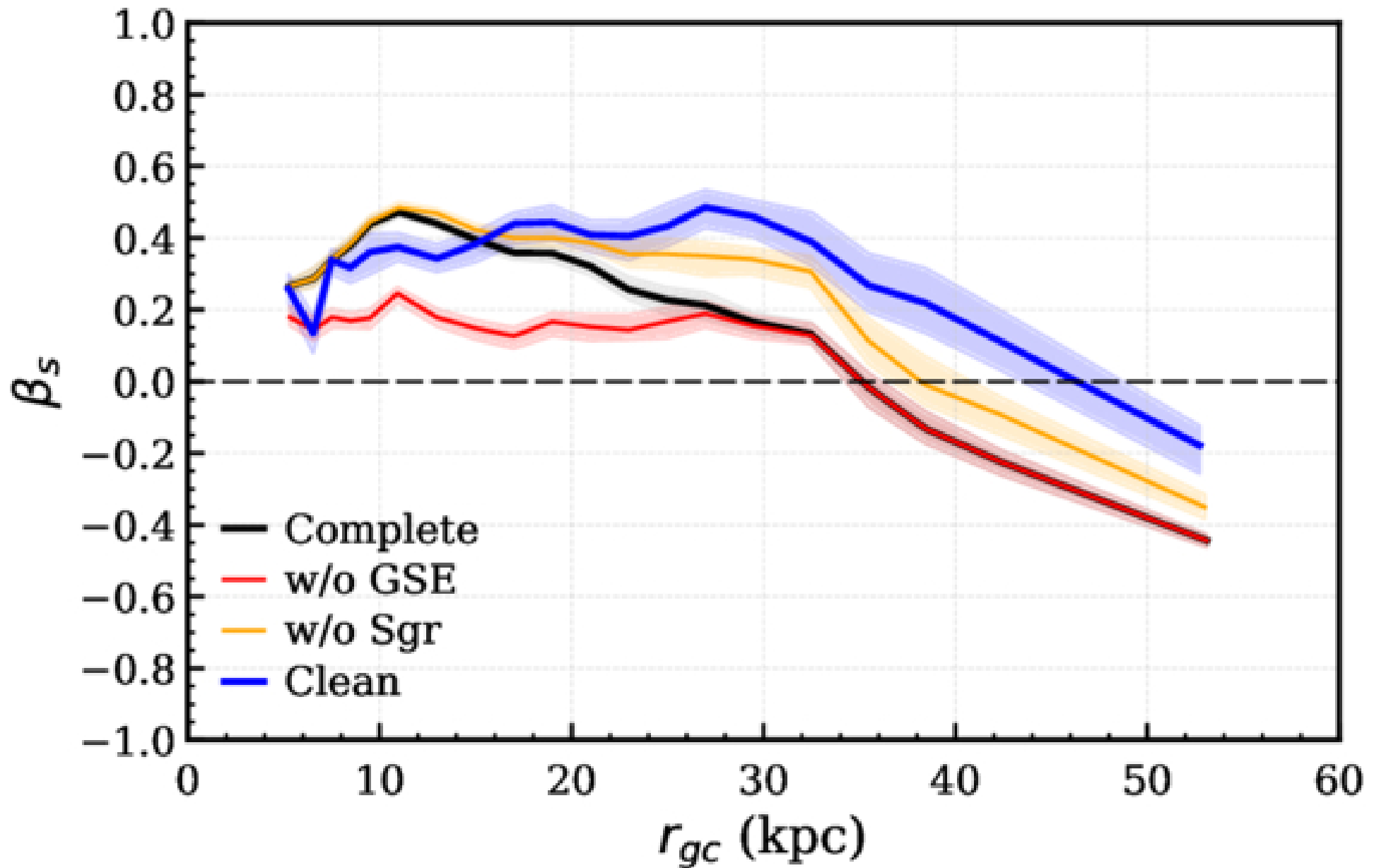
Figure 5. from F. O. Barbosa et al 2026 Astrophys. J. 1008 doi:10.3847/1538-4357/ae8fd6 https://dx.doi.org/10.3847/1538-4357/ae8fd6 © 2026. The Author(s). Published by the American Astronomical Society.
