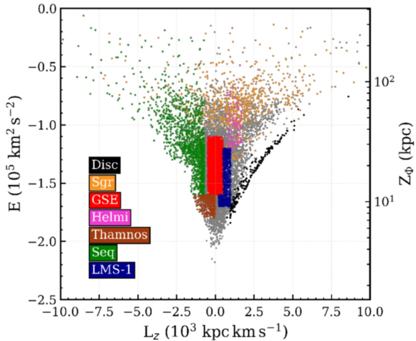
Figure 2. from F. O. Barbosa et al 2026 Astrophys. J. 1008 doi:10.3847/1538-4357/ae8fd6 https://dx.doi.org/10.3847/1538-4357/ae8fd6 © 2026. The Author(s). Published by the American Astronomical Society.
