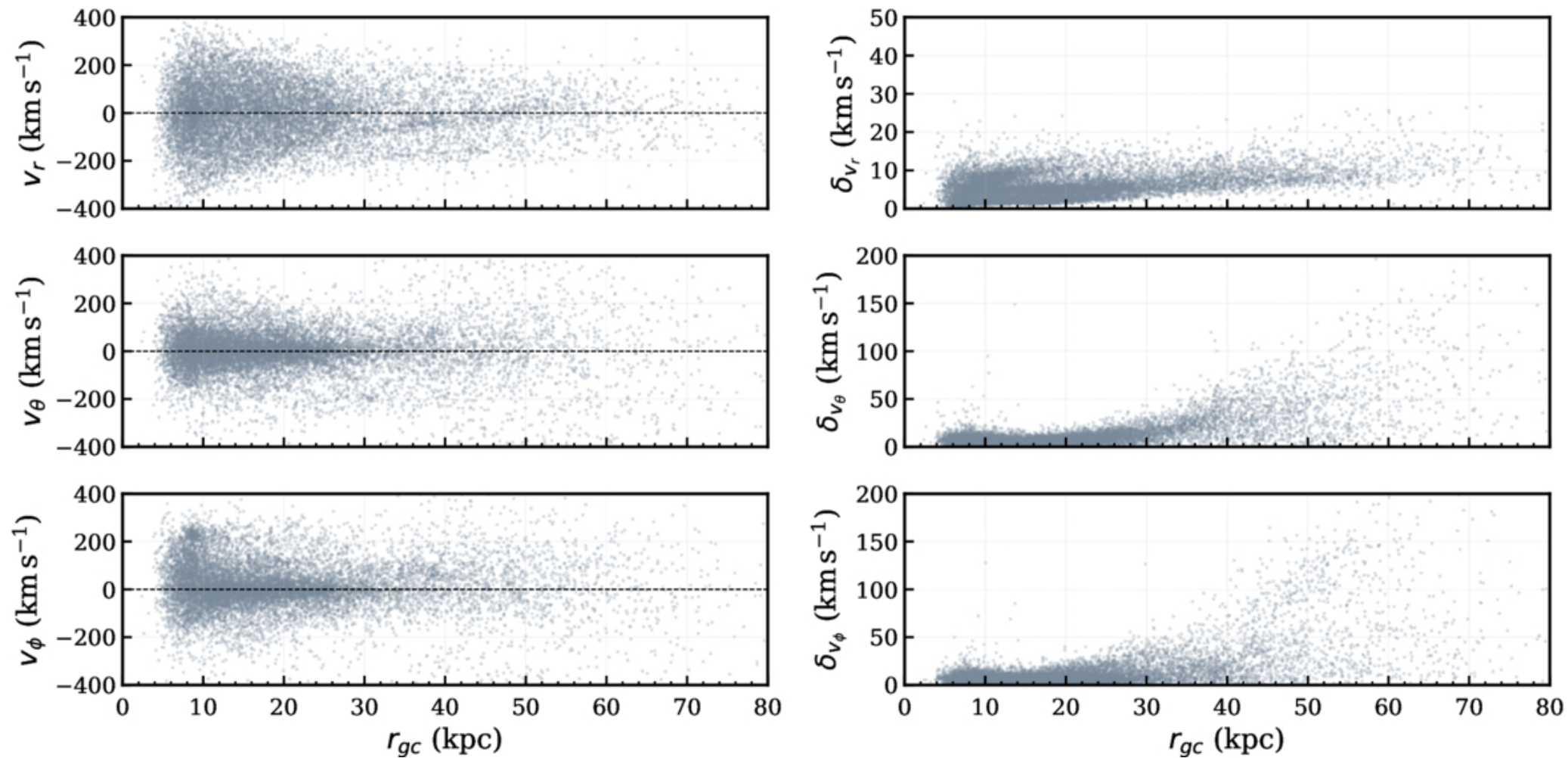
Figure 1. from F. O. Barbosa et al 2026 Astrophys. J. 1008 doi:10.3847/1538-4357/ae8fd6 https://dx.doi.org/10.3847/1538-4357/ae8fd6 © 2026. The Author(s). Published by the American Astronomical Society.
