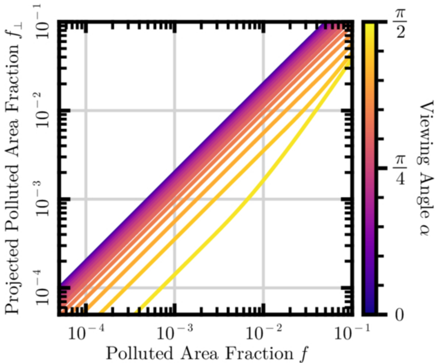
Figure 9. from Dang Pham et al 2026 Astrophys. J. 1008 doi:10.3847/1538-4357/ae8fd5 https://dx.doi.org/10.3847/1538-4357/ae8fd5 © 2026. The Author(s). Published by the American Astronomical Society.
