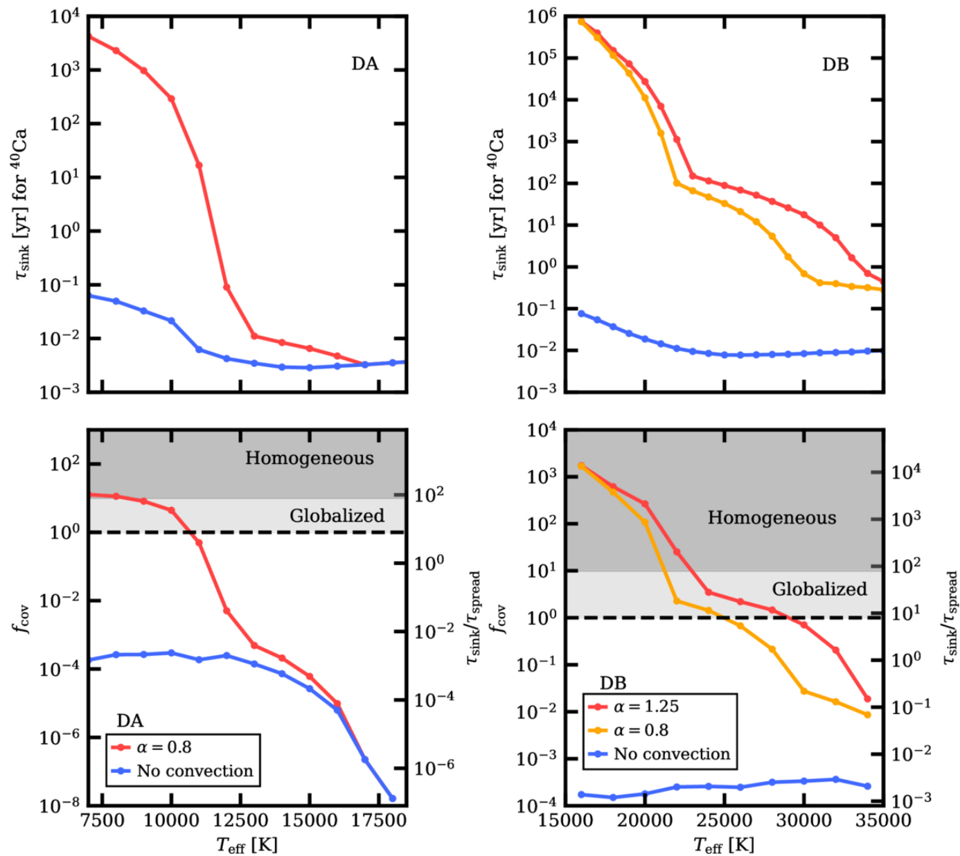
Figure 8. from Dang Pham et al 2026 Astrophys. J. 1008 doi:10.3847/1538-4357/ae8fd5 https://dx.doi.org/10.3847/1538-4357/ae8fd5 © 2026. The Author(s). Published by the American Astronomical Society.
