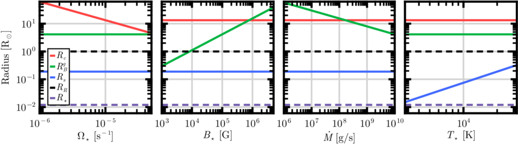
Figure 2. from Dang Pham et al 2026 Astrophys. J. 1008 doi:10.3847/1538-4357/ae8fd5 https://dx.doi.org/10.3847/1538-4357/ae8fd5 © 2026. The Author(s). Published by the American Astronomical Society.
