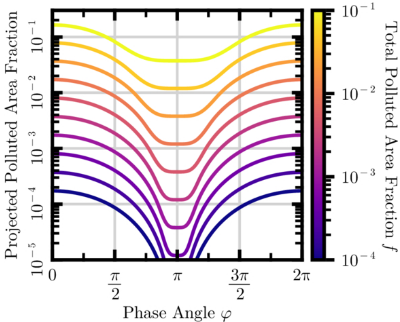
Figure 10. from Dang Pham et al 2026 Astrophys. J. 1008 doi:10.3847/1538-4357/ae8fd5 https://dx.doi.org/10.3847/1538-4357/ae8fd5 © 2026. The Author(s). Published by the American Astronomical Society.
