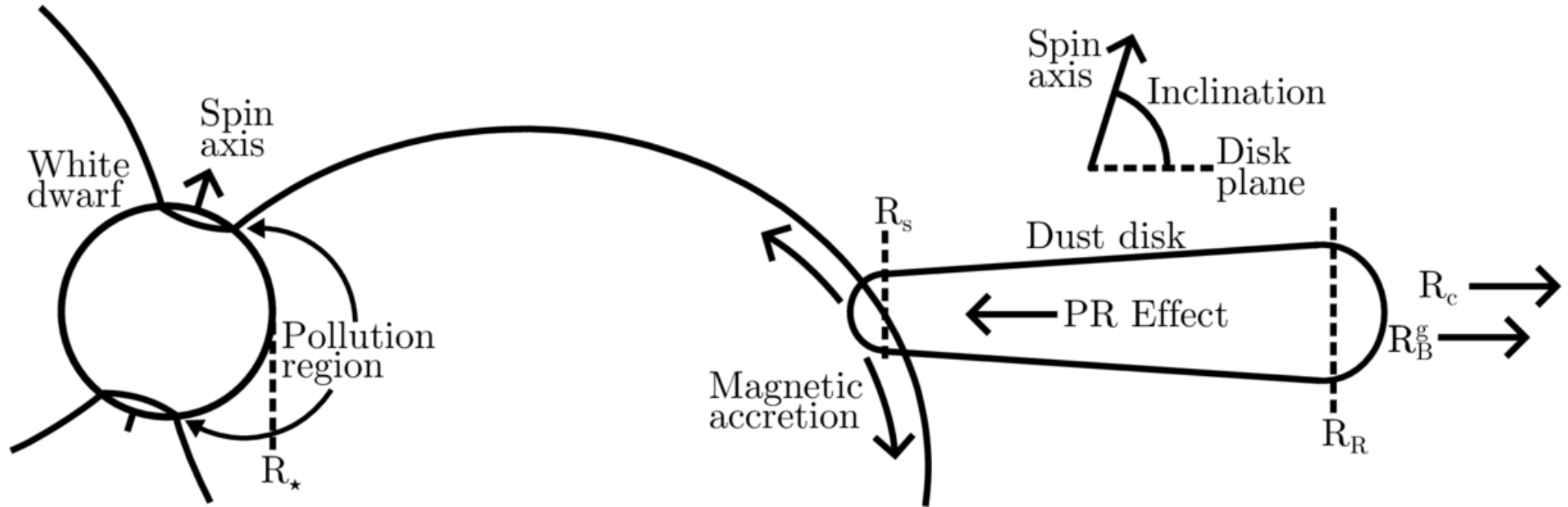
Figure 1. from Dang Pham et al 2026 Astrophys. J. 1008 doi:10.3847/1538-4357/ae8fd5 https://dx.doi.org/10.3847/1538-4357/ae8fd5 © 2026. The Author(s). Published by the American Astronomical Society.
