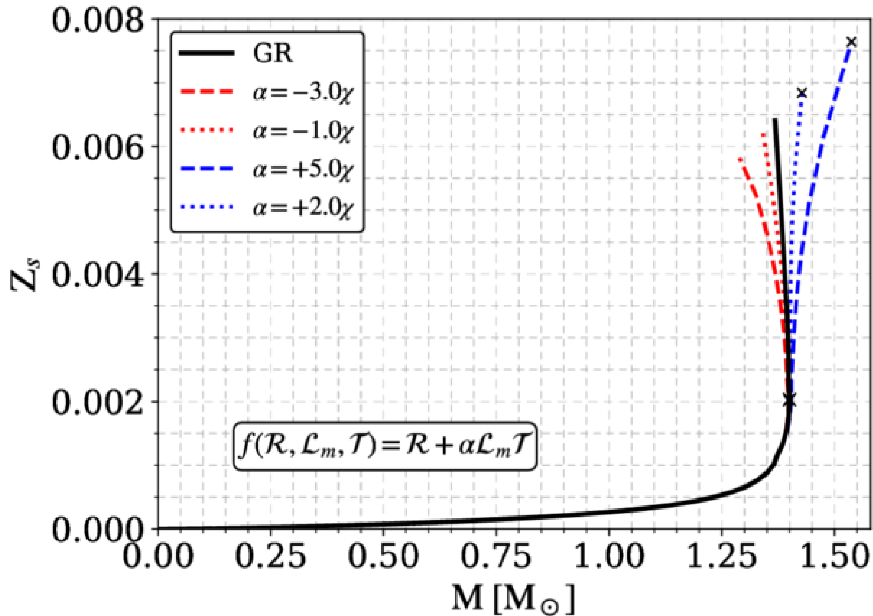
Figure 7. from N. Priyobarta et al 2026 Astrophys. J. 1007 doi:10.3847/1538-4357/ae8fd2 https://dx.doi.org/10.3847/1538-4357/ae8fd2 © 2026. The Author(s). Published by the American Astronomical Society.
