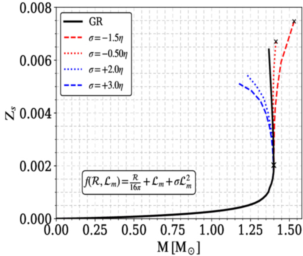
Figure 6. from N. Priyobarta et al 2026 Astrophys. J. 1007 doi:10.3847/1538-4357/ae8fd2 https://dx.doi.org/10.3847/1538-4357/ae8fd2 © 2026. The Author(s). Published by the American Astronomical Society.
