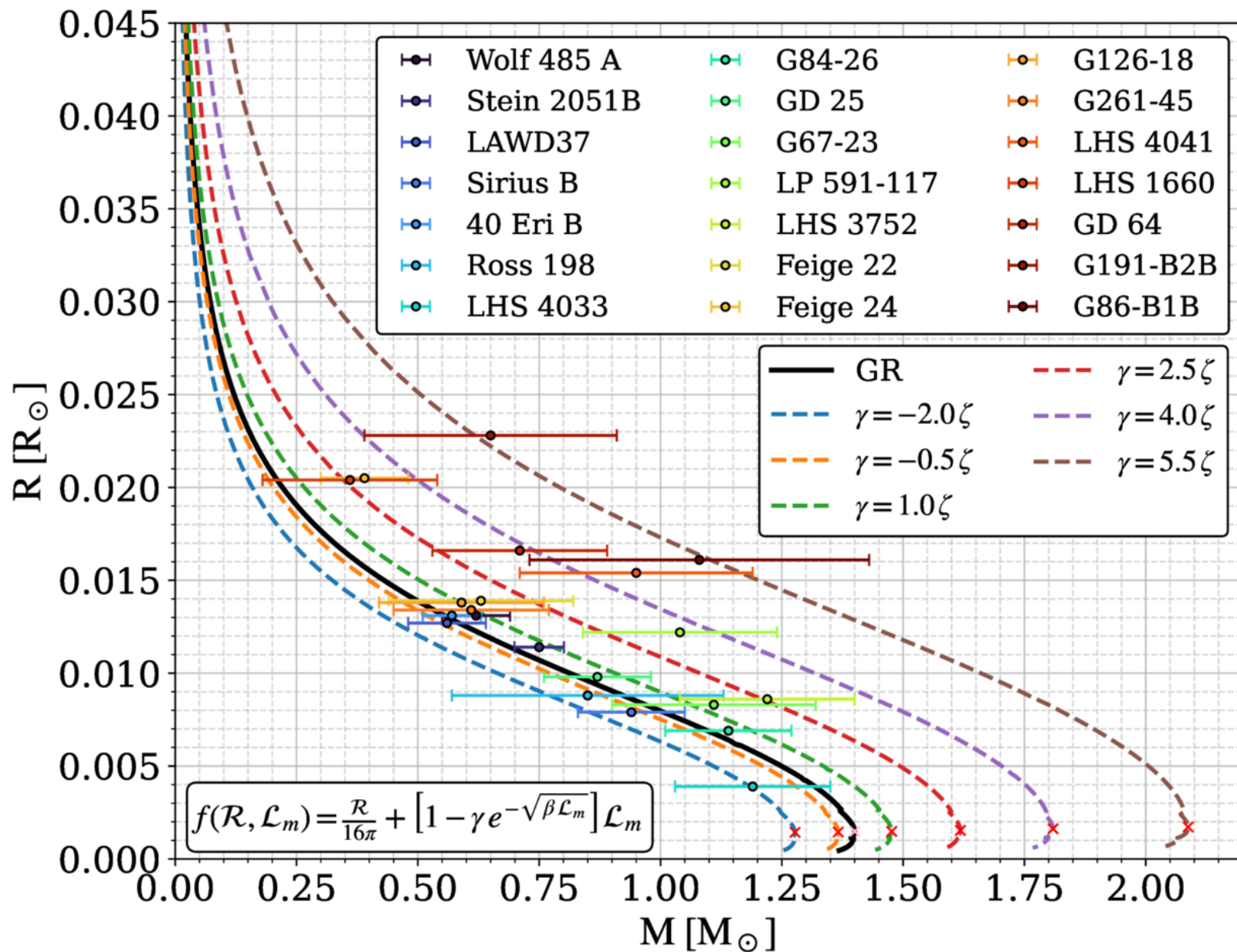
Figure 2. from N. Priyobarta et al 2026 Astrophys. J. 1007 doi:10.3847/1538-4357/ae8fd2 https://dx.doi.org/10.3847/1538-4357/ae8fd2 © 2026. The Author(s). Published by the American Astronomical Society.
