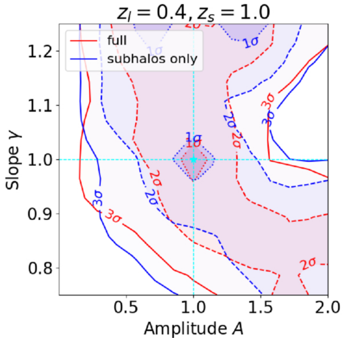
Figure 7. from Andreas Filipp et al 2026 Astrophys. J. 1007 doi:10.3847/1538-4357/ae8fd0 https://dx.doi.org/10.3847/1538-4357/ae8fd0 © 2026. The Author(s). Published by the American Astronomical Society.
