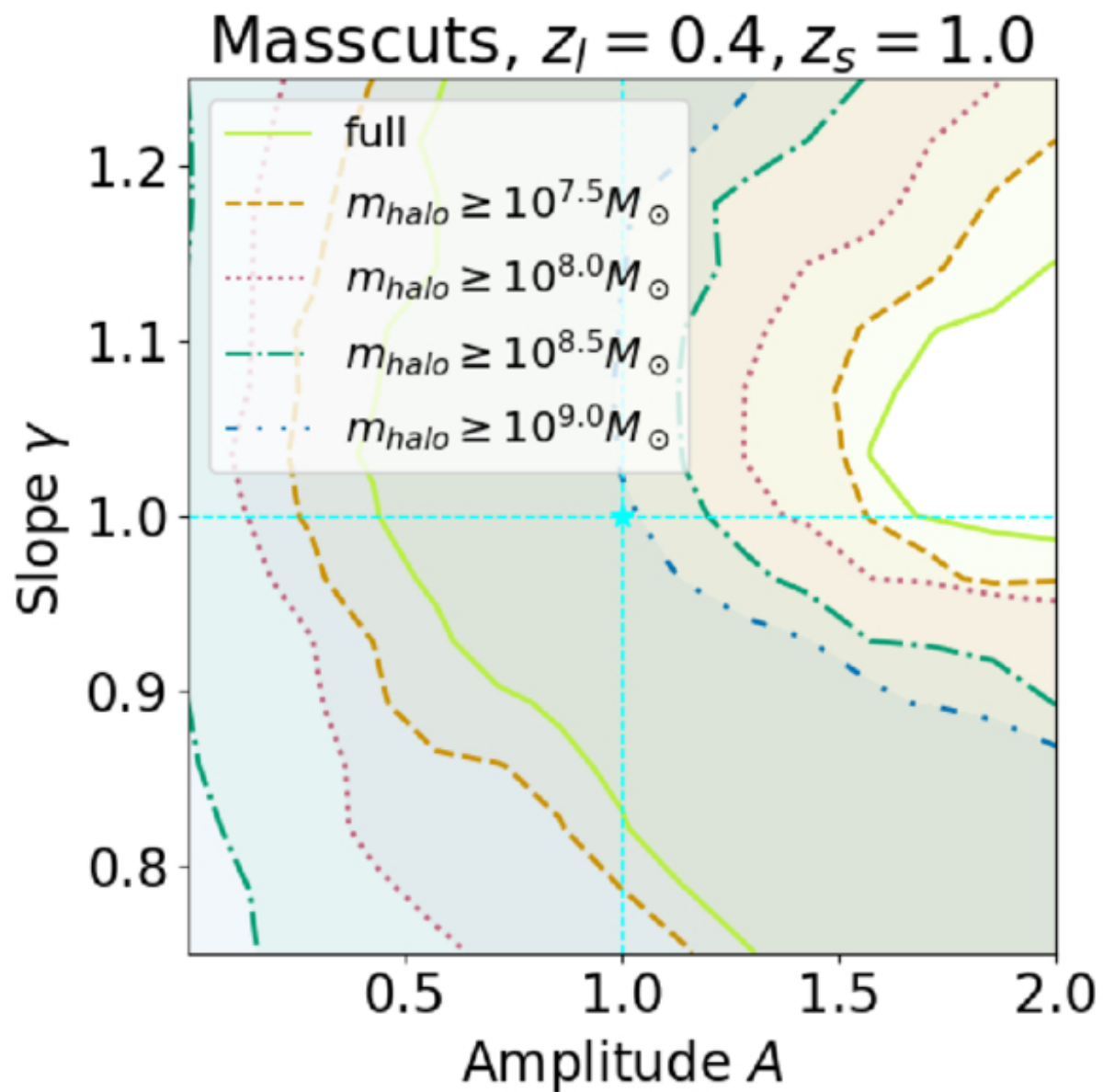
Figure 6. from Andreas Filipp et al 2026 Astrophys. J. 1007 doi:10.3847/1538-4357/ae8fd0 https://dx.doi.org/10.3847/1538-4357/ae8fd0 © 2026. The Author(s). Published by the American Astronomical Society.
