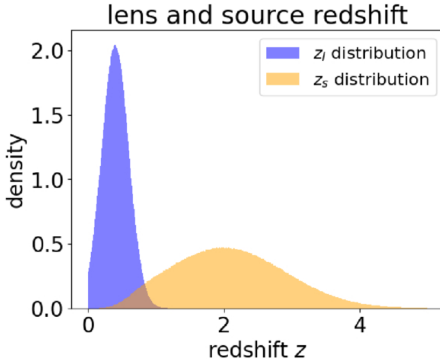
Figure 3. from Andreas Filipp et al 2026 Astrophys. J. 1007 doi:10.3847/1538-4357/ae8fd0 https://dx.doi.org/10.3847/1538-4357/ae8fd0 © 2026. The Author(s). Published by the American Astronomical Society.
