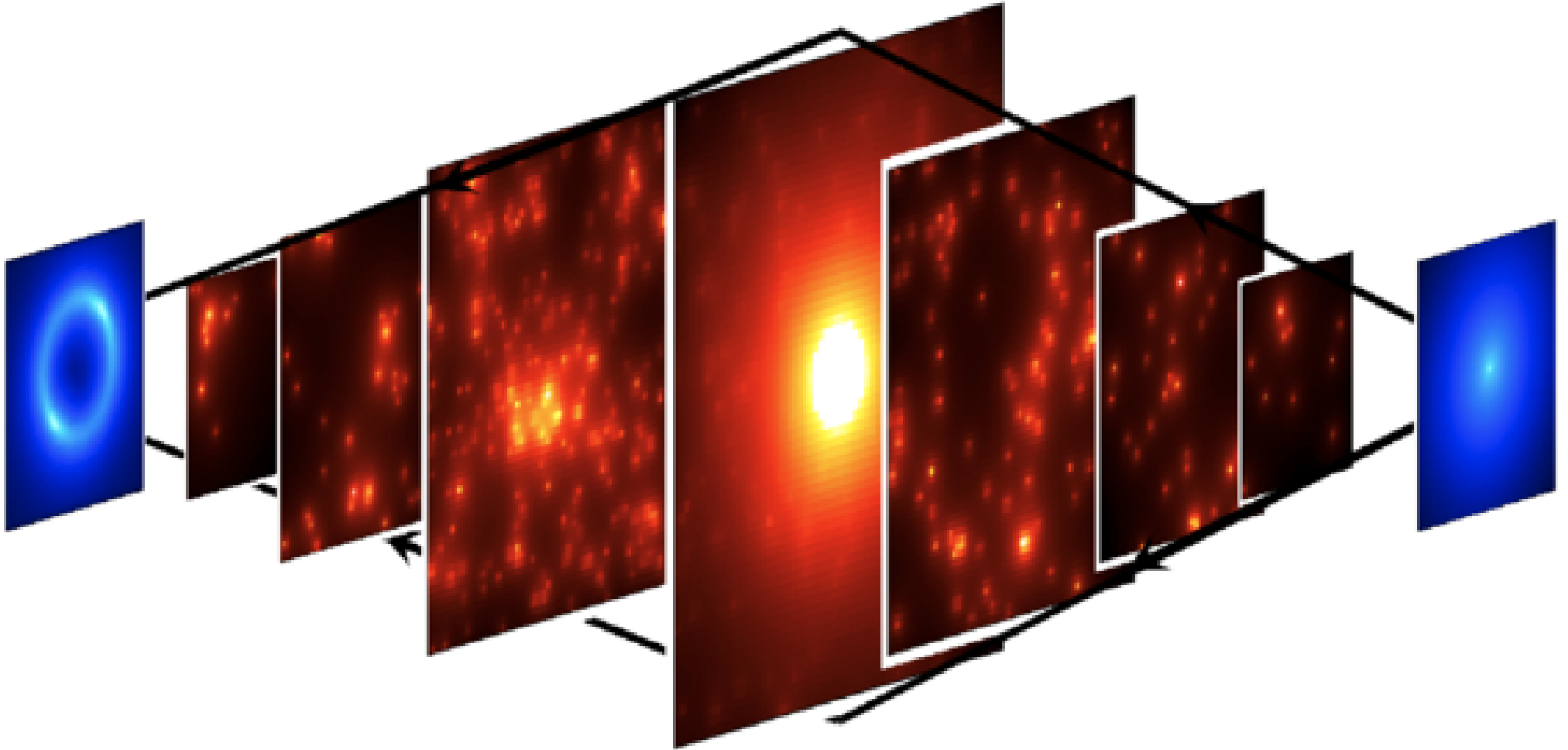
Figure 2. from Andreas Filipp et al 2026 Astrophys. J. 1007 doi:10.3847/1538-4357/ae8fd0 https://dx.doi.org/10.3847/1538-4357/ae8fd0 © 2026. The Author(s). Published by the American Astronomical Society.
