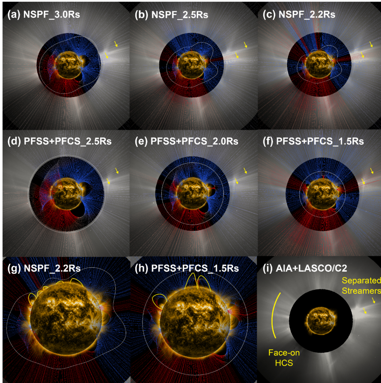
Figure 3. from Ziqi Wu et al 2026 Astrophys. J. 1007 doi:10.3847/1538-4357/ae8f45 https://dx.doi.org/10.3847/1538-4357/ae8f45 © 2026. The Author(s). Published by the American Astronomical Society.
