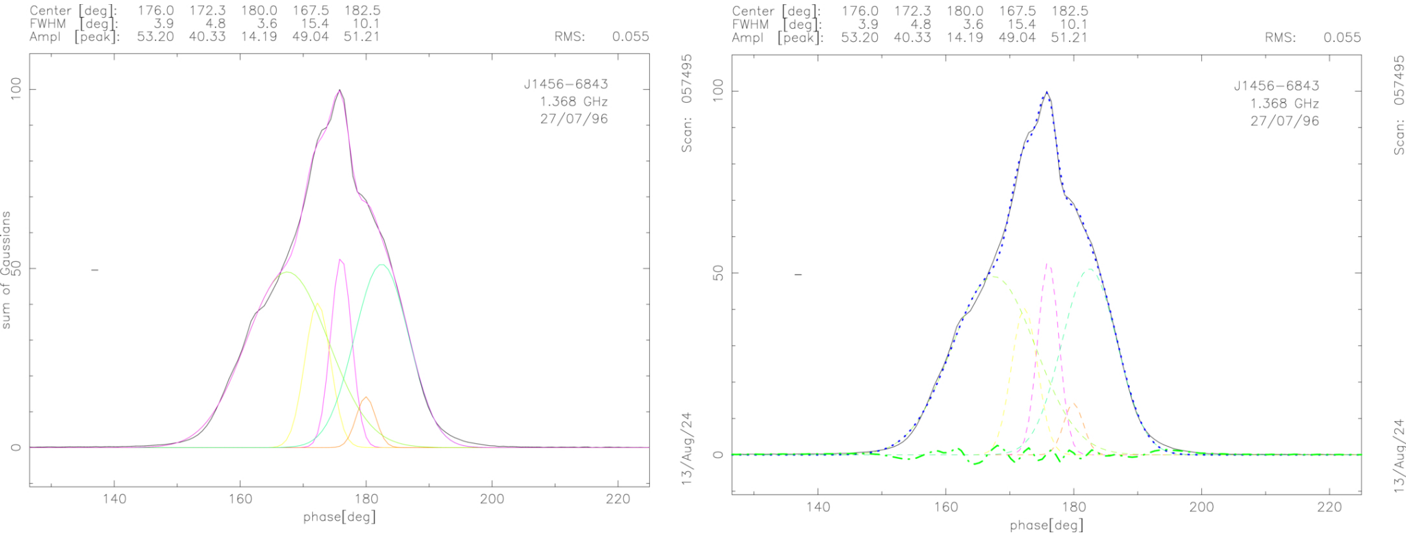
Figure A2. from N. D. Ramesh Bhat et al 2026 Astrophys. J. 1010 doi:10.3847/1538-4357/ae8f3e https://dx.doi.org/10.3847/1538-4357/ae8f3e © 2026. The Author(s). Published by the American Astronomical Society.
