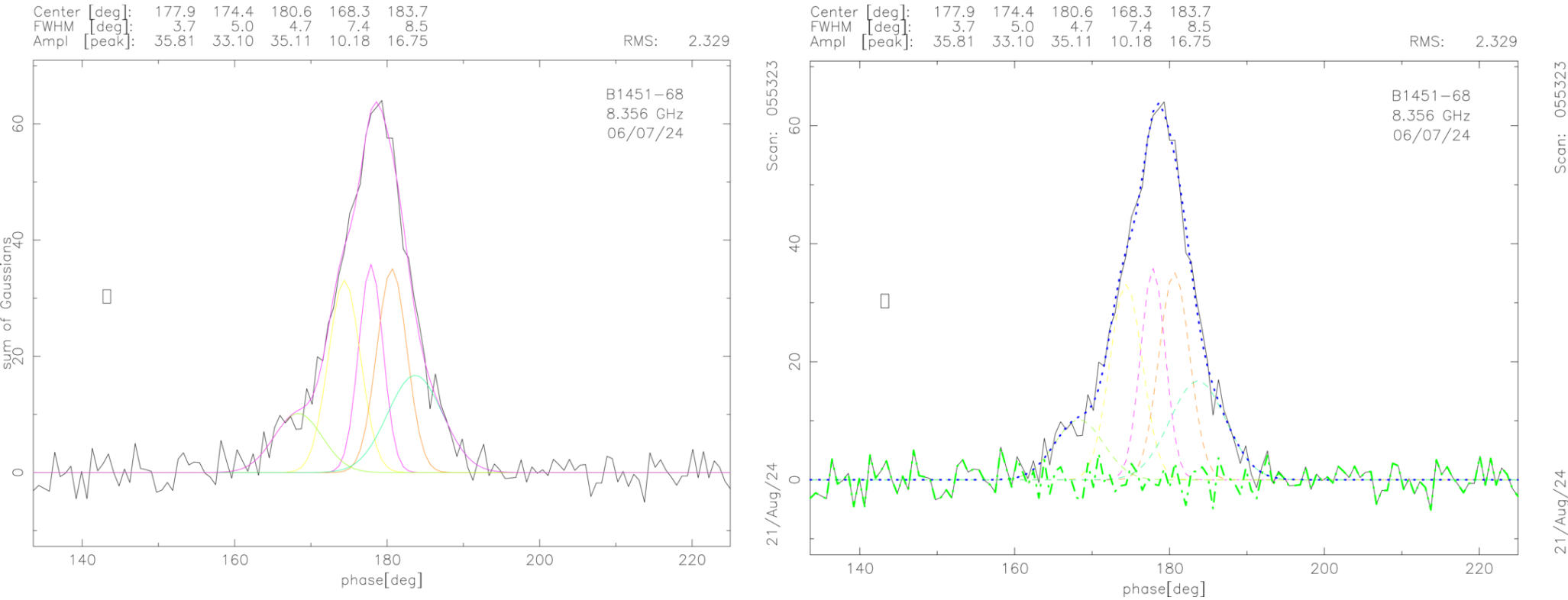
Figure A1. from N. D. Ramesh Bhat et al 2026 Astrophys. J. 1010 doi:10.3847/1538-4357/ae8f3e https://dx.doi.org/10.3847/1538-4357/ae8f3e © 2026. The Author(s). Published by the American Astronomical Society.
