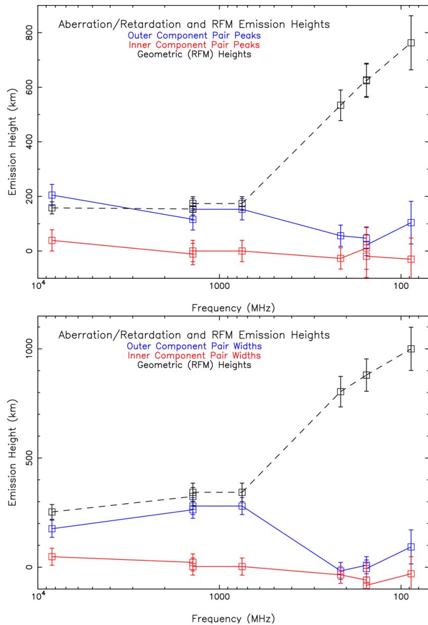
Figure 4. from N. D. Ramesh Bhat et al 2026 Astrophys. J. 1010 doi:10.3847/1538-4357/ae8f3e https://dx.doi.org/10.3847/1538-4357/ae8f3e © 2026. The Author(s). Published by the American Astronomical Society.
