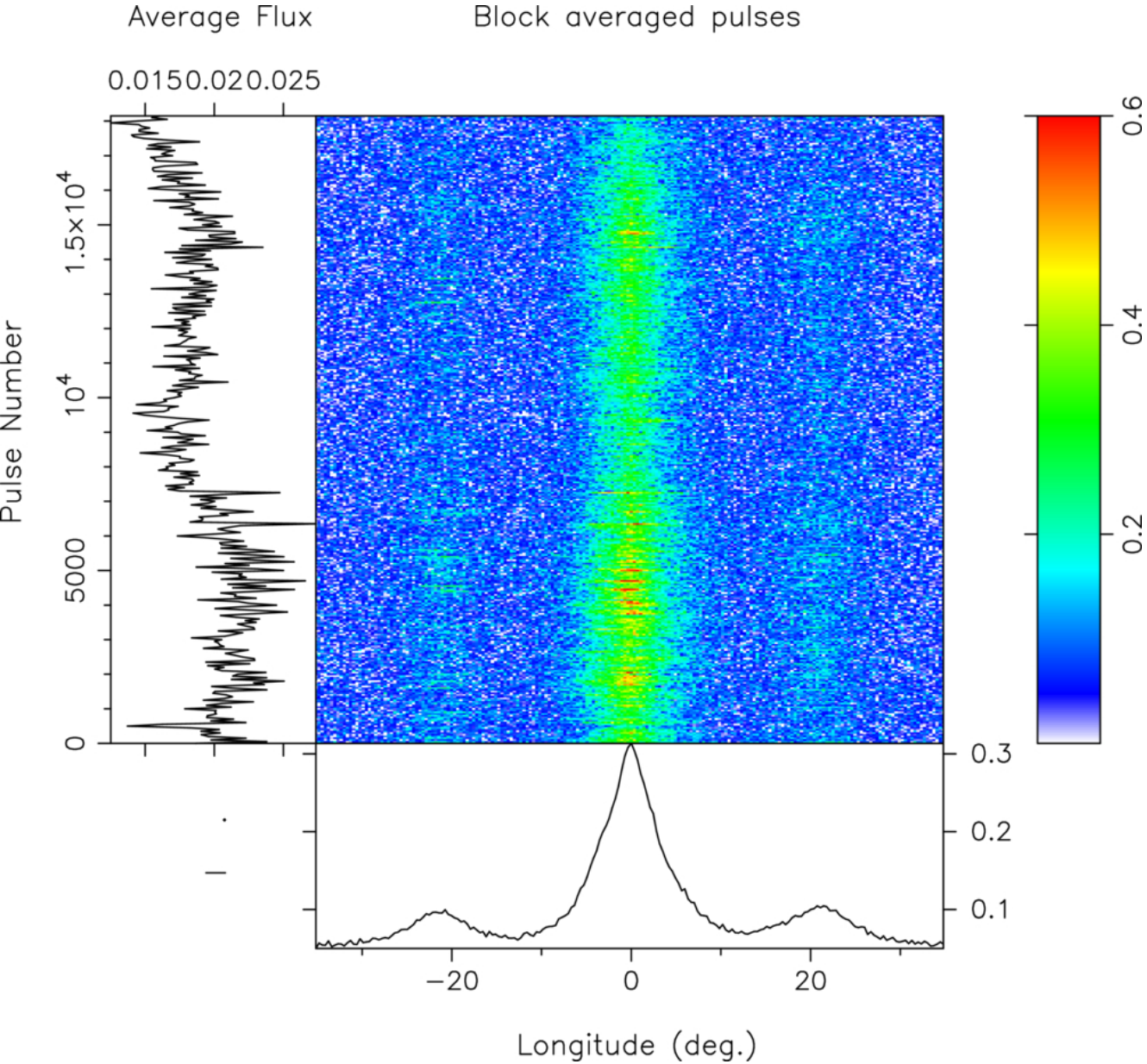
Figure 2. from N. D. Ramesh Bhat et al 2026 Astrophys. J. 1010 doi:10.3847/1538-4357/ae8f3e https://dx.doi.org/10.3847/1538-4357/ae8f3e © 2026. The Author(s). Published by the American Astronomical Society.
