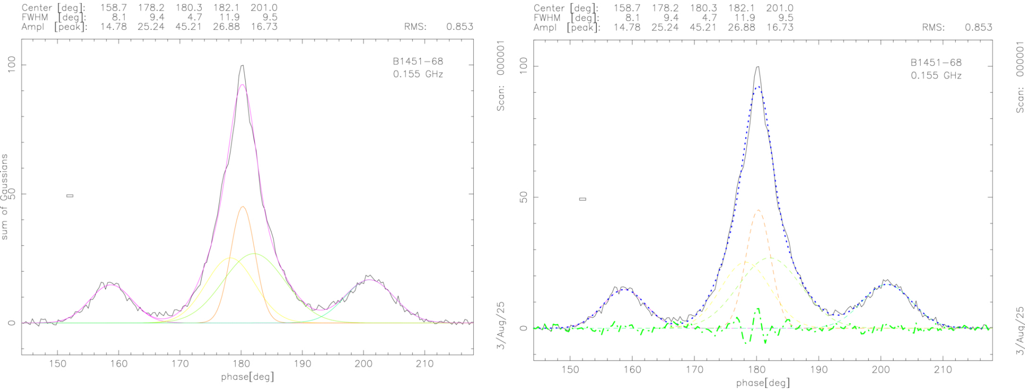
Figure A7. from N. D. Ramesh Bhat et al 2026 Astrophys. J. 1010 doi:10.3847/1538-4357/ae8f3e https://dx.doi.org/10.3847/1538-4357/ae8f3e © 2026. The Author(s). Published by the American Astronomical Society.
