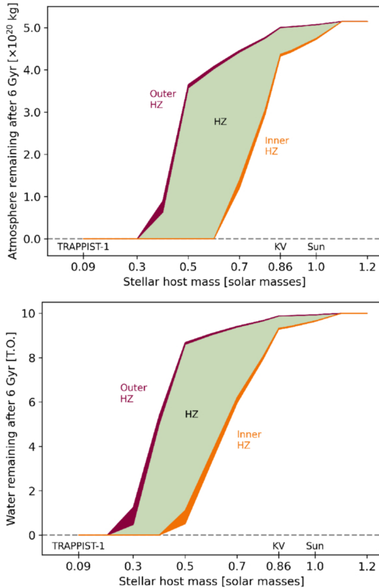
Figure 6. from Nathaniel Tanglin and Juliette Becker 2026 Astrophys. J. 1008 doi:10.3847/1538-4357/ae8f2b https://dx.doi.org/10.3847/1538-4357/ae8f2b © 2026. The Author(s). Published by the American Astronomical Society.
